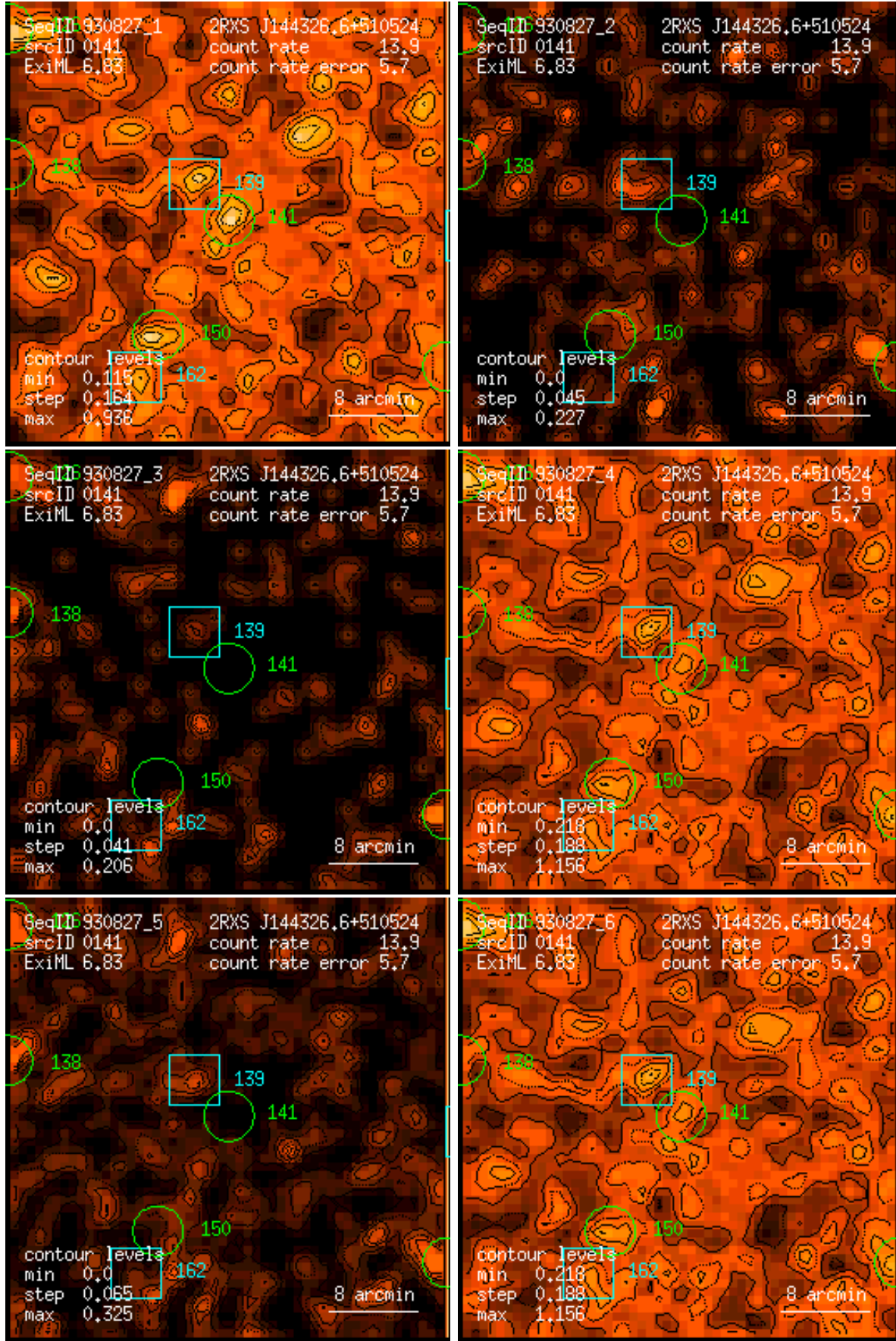
Figure 141: RASS 930827: detection 0141: band rate images, Gaussian filter: (1) PSPC channels 11 – 41, (2) 52 – 90, (3) 91 – 201, (4) 11 – 235, (5) 52 – 201, (6) 11 – 201. Broad band rates in counts/ks. Band rate contour levels in counts/ks/arcmin 2 .
