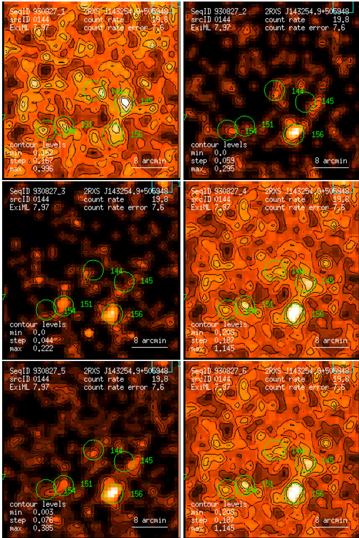
Figure 144: RASS 930827: detection 0144: band rate images, Gaussian filter: (1) PSPC channels 11 – 41, (2) 52 – 90, (3) 91 – 201, (4) 11 – 235, (5) 52 – 201, (6) 11 – 201. Broad band rates in counts/ks. Band rate contour levels in counts/ks/arcmin 2 .
