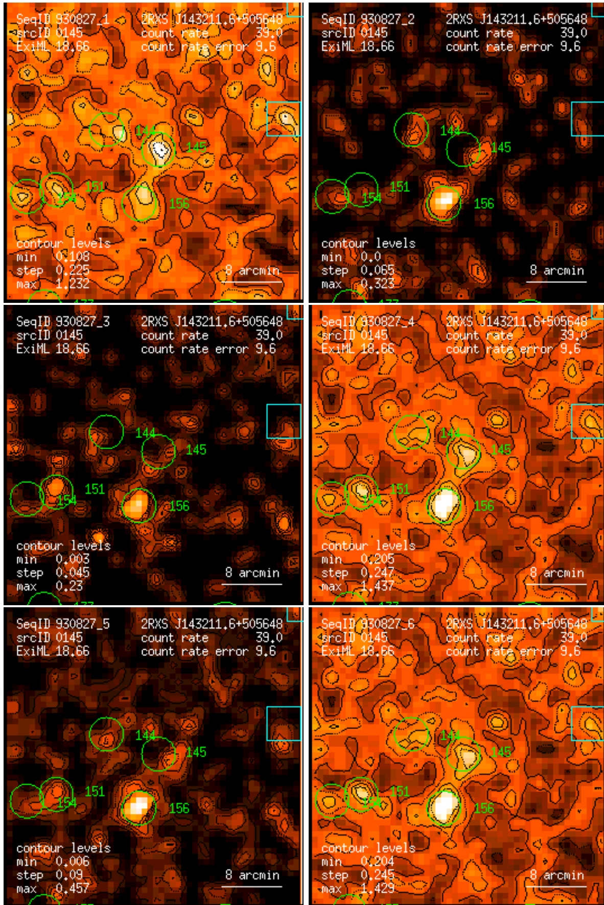
Figure 145: RASS 930827: detection 0145: band rate images, Gaussian filter: (1) PSPC channels 11 – 41, (2) 52 – 90, (3) 91 – 201, (4) 11 – 235, (5) 52 – 201, (6) 11 – 201. Broad band rates in counts/ks. Band rate contour levels in counts/ks/arcmin 2 .
