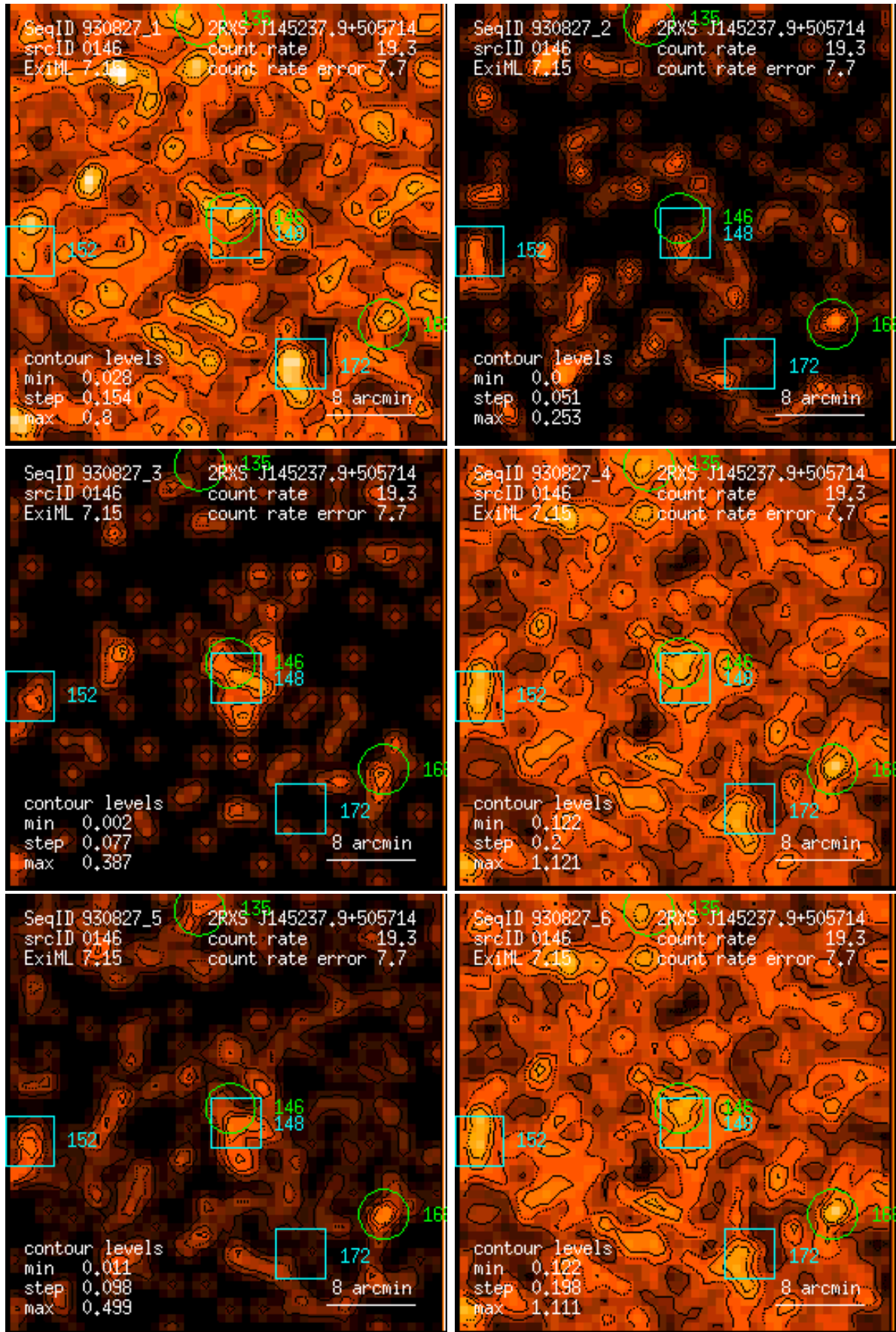
Figure 146: RASS 930827: detection 0146: band rate images, Gaussian filter: (1) PSPC channels 11 – 41, (2) 52 – 90, (3) 91 – 201, (4) 11 – 235, (5) 52 – 201, (6) 11 – 201. Broad band rates in counts/ks. Band rate contour levels in counts/ks/arcmin 2 .
