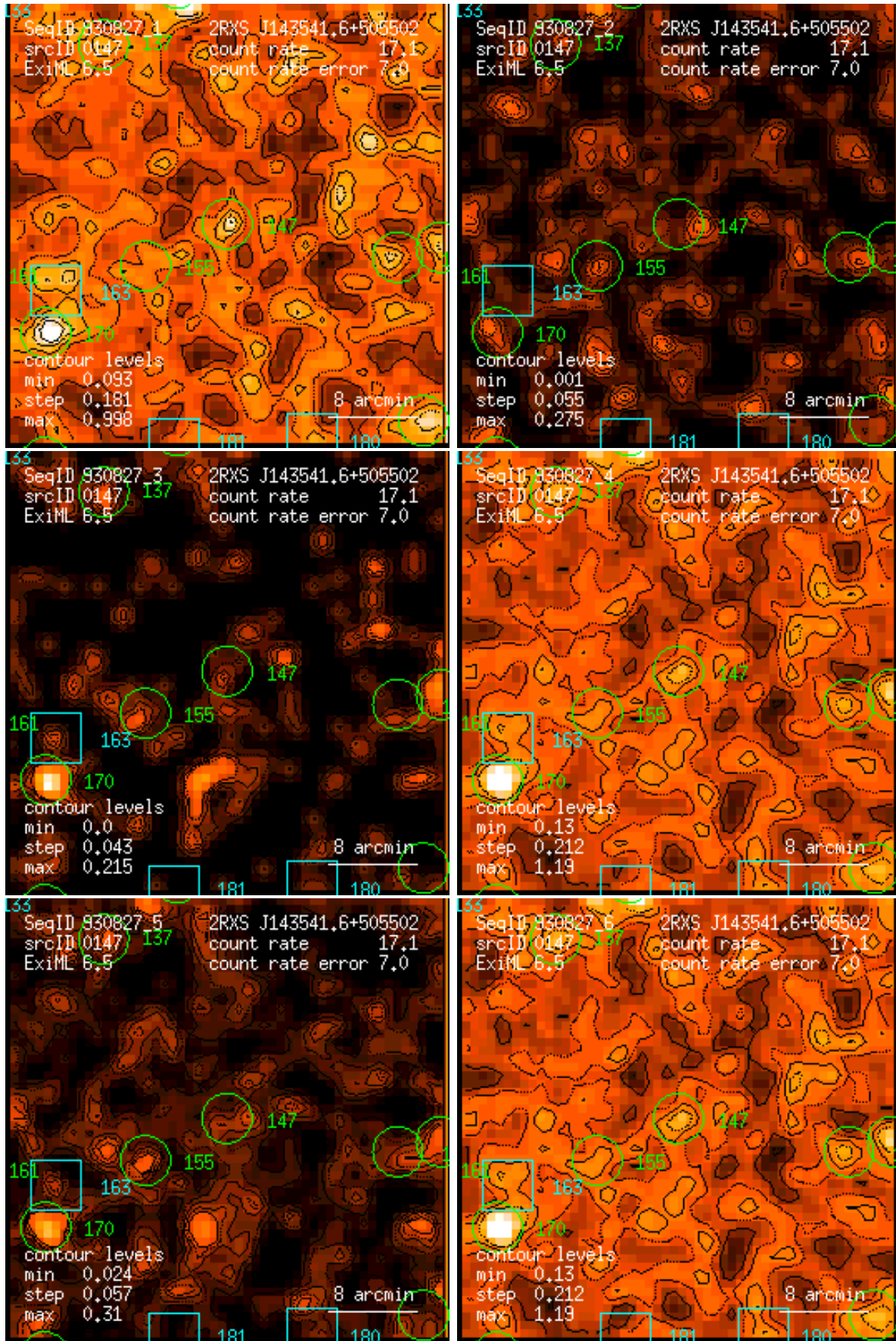
Figure 147: RASS 930827: detection 0147: band rate images, Gaussian filter: (1) PSPC channels 11 – 41, (2) 52 – 90, (3) 91 – 201, (4) 11 – 235, (5) 52 – 201, (6) 11 – 201. Broad band rates in counts/ks. Band rate contour levels in counts/ks/arcmin 2 .
