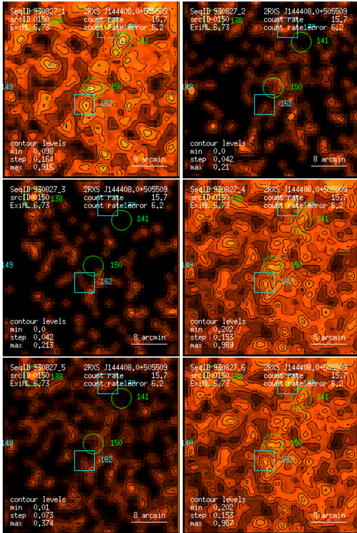
Figure 150: RASS 930827: detection 0150: band rate images, Gaussian filter: (1) PSPC channels 11 – 41, (2) 52 – 90, (3) 91 – 201, (4) 11 – 235, (5) 52 – 201, (6) 11 – 201. Broad band rates in counts/ks. Band rate contour levels in counts/ks/arcmin 2 .
