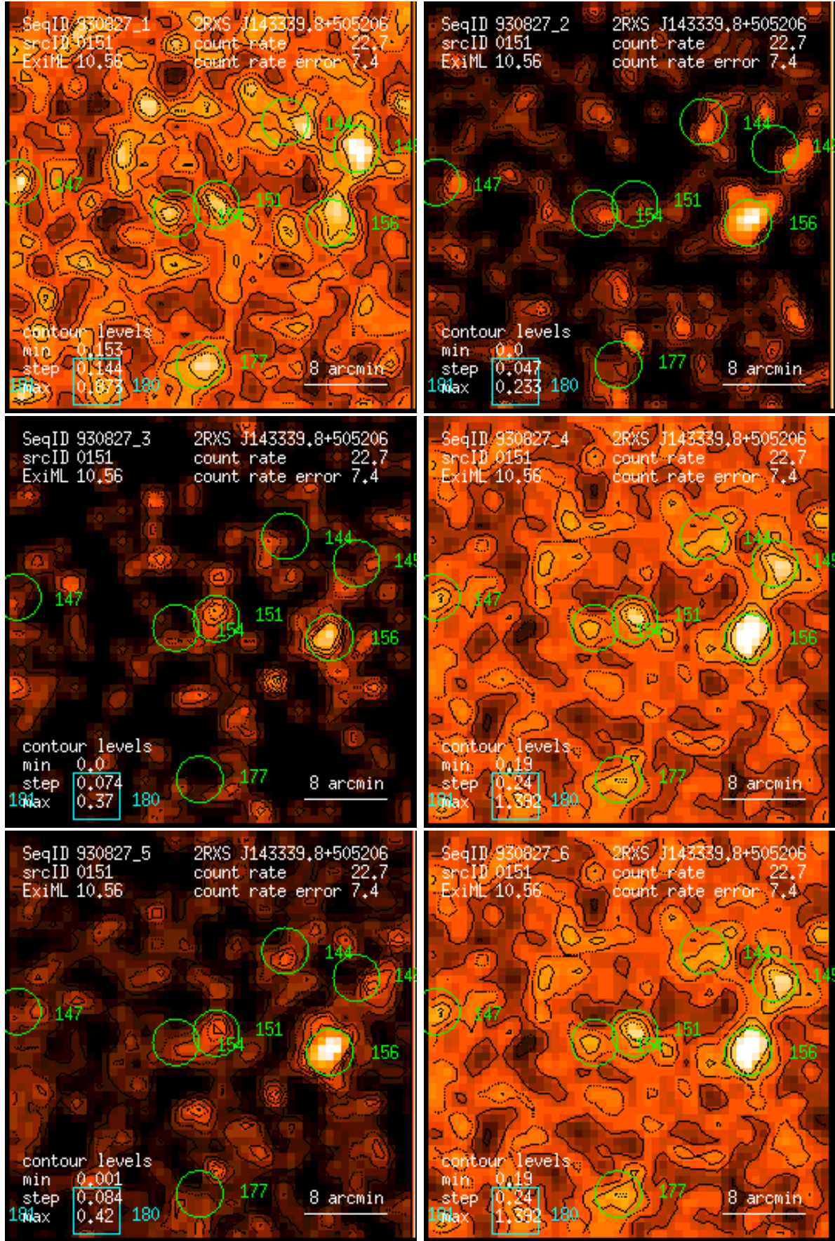
Figure 151: RASS 930827: detection 0151: band rate images, Gaussian filter: (1) PSPC channels 11 – 41, (2) 52 – 90, (3) 91 – 201, (4) 11 – 235, (5) 52 – 201, (6) 11 – 201. Broad band rates in counts/ks. Band rate contour levels in counts/ks/arcmin 2 .
