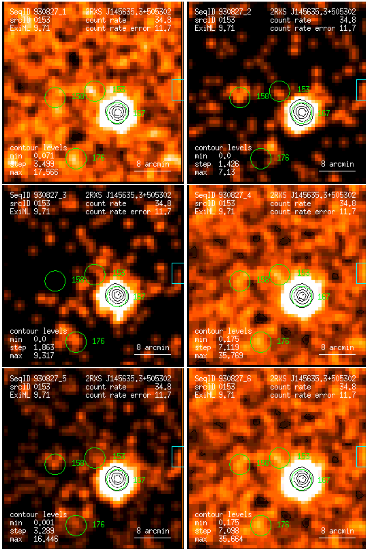
Figure 153: RASS 930827: detection 0153: band rate images, Gaussian filter: (1) PSPC channels 11 – 41, (2) 52 – 90, (3) 91 – 201, (4) 11 – 235, (5) 52 – 201, (6) 11 – 201. Broad band rates in counts/ks. Band rate contour levels in counts/ks/arcmin 2 .
