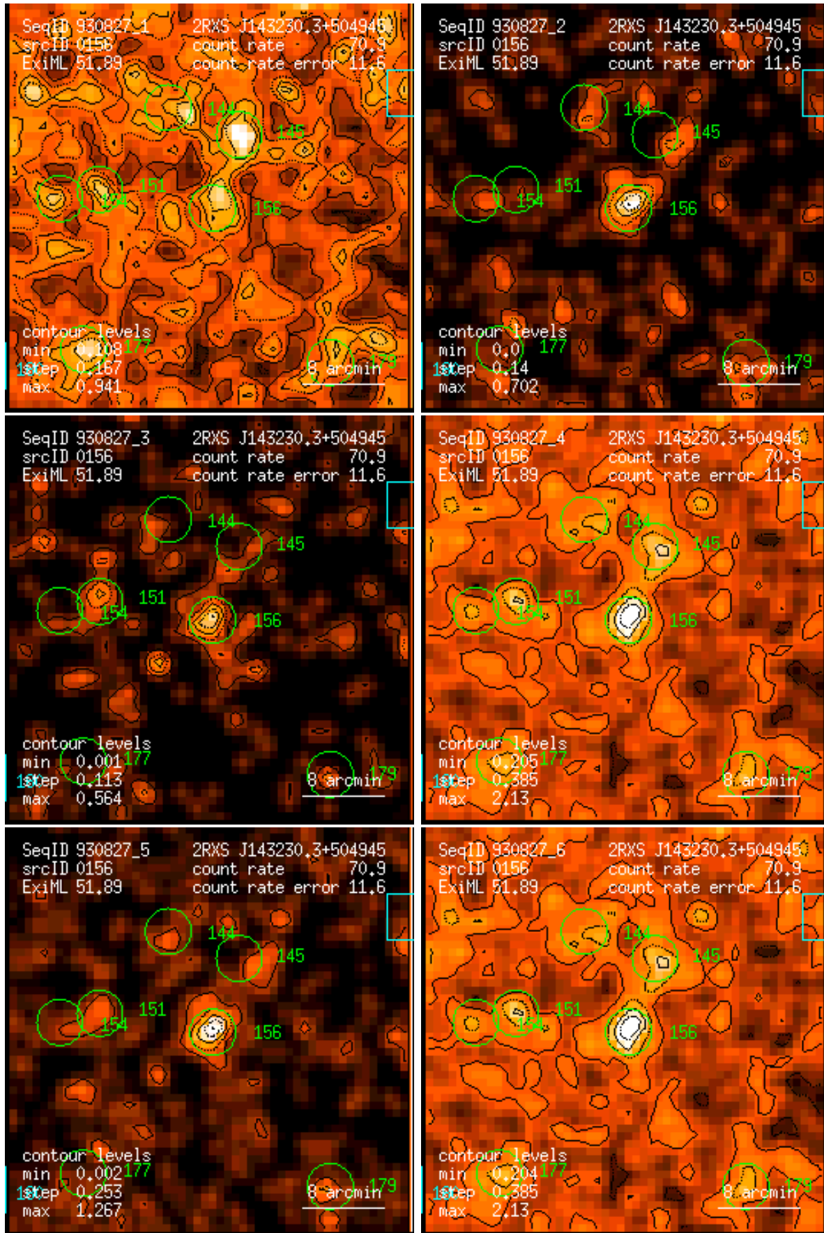
Figure 156: RASS 930827: detection 0156: band rate images, Gaussian filter: (1) PSPC channels 11 – 41, (2) 52 – 90, (3) 91 – 201, (4) 11 – 235, (5) 52 – 201, (6) 11 – 201. Broad band rates in counts/ks. Band rate contour levels in counts/ks/arcmin 2 .
