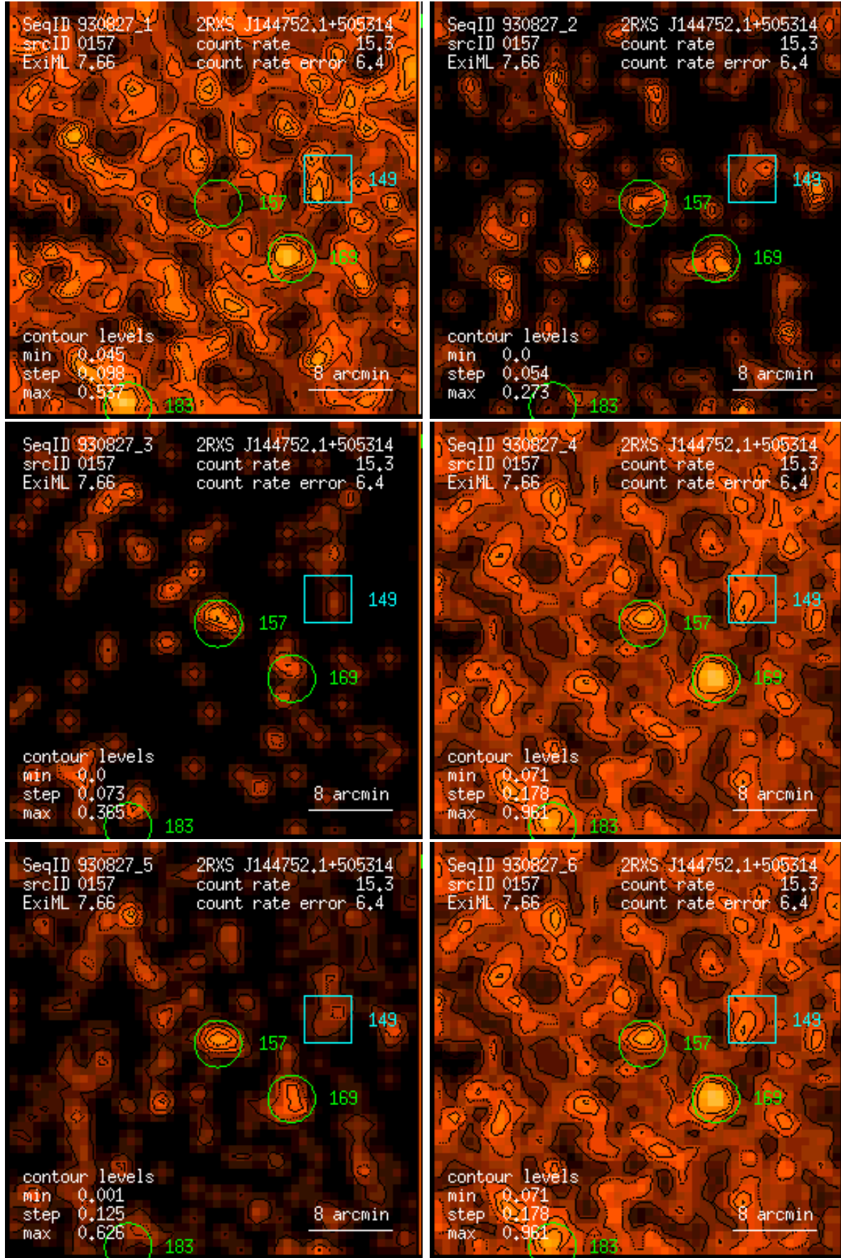
Figure 157: RASS 930827: detection 0157: band rate images, Gaussian filter: (1) PSPC channels 11 – 41, (2) 52 – 90, (3) 91 – 201, (4) 11 – 235, (5) 52 – 201, (6) 11 – 201. Broad band rates in counts/ks. Band rate contour levels in counts/ks/arcmin 2 .
