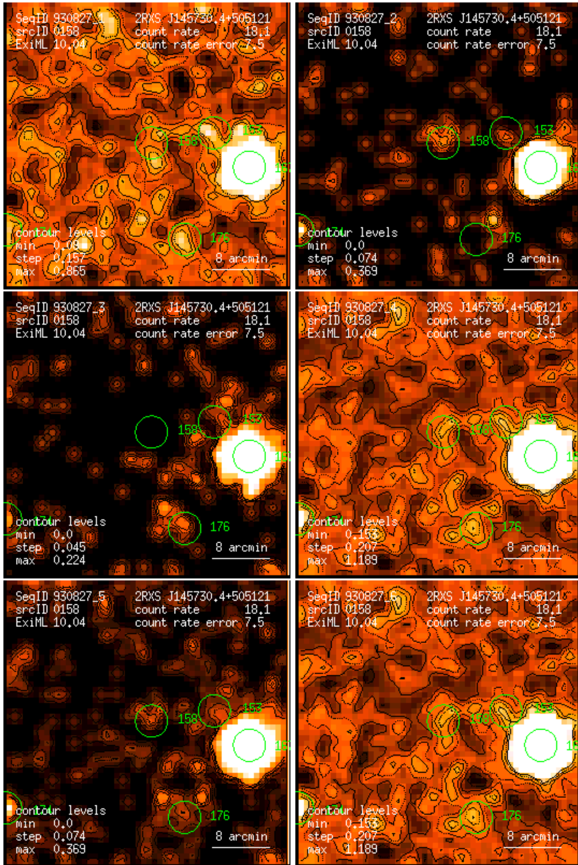
Figure 158: RASS 930827: detection 0158: band rate images, Gaussian filter: (1) PSPC channels 11 – 41, (2) 52 – 90, (3) 91 – 201, (4) 11 – 235, (5) 52 – 201, (6) 11 – 201. Broad band rates in counts/ks. Band rate contour levels in counts/ks/arcmin 2 .
