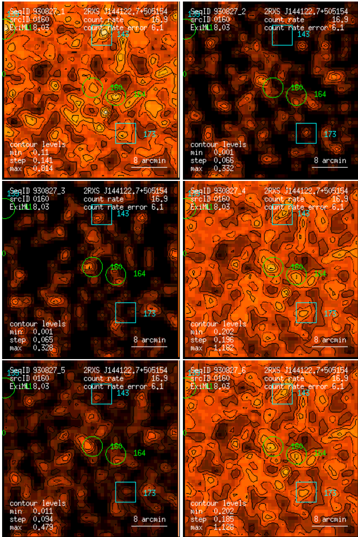
Figure 160: RASS 930827: detection 0160: band rate images, Gaussian filter: (1) PSPC channels 11 – 41, (2) 52 – 90, (3) 91 – 201, (4) 11 – 235, (5) 52 – 201, (6) 11 – 201. Broad band rates in counts/ks. Band rate contour levels in counts/ks/arcmin 2 .
