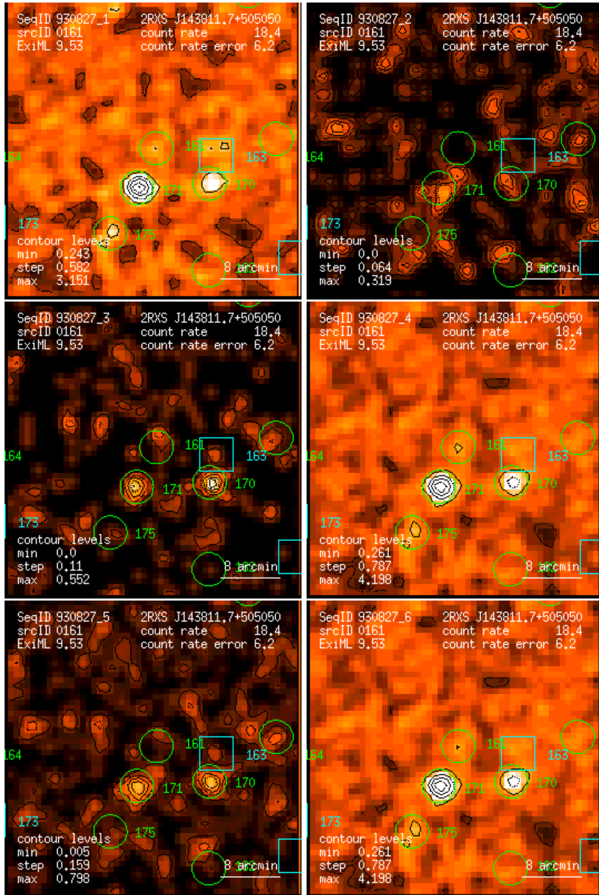
Figure 161: RASS 930827: detection 0161: band rate images, Gaussian filter: (1) PSPC channels 11 – 41, (2) 52 – 90, (3) 91 – 201, (4) 11 – 235, (5) 52 – 201, (6) 11 – 201. Broad band rates in counts/ks. Band rate contour levels in counts/ks/arcmin 2 .
