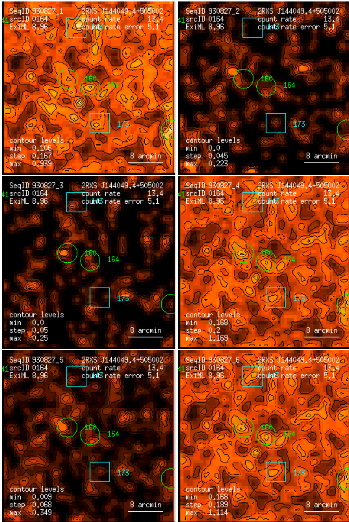
Figure 164: RASS 930827: detection 0164: band rate images, Gaussian filter: (1) PSPC channels 11 – 41, (2) 52 – 90, (3) 91 – 201, (4) 11 – 235, (5) 52 – 201, (6) 11 – 201. Broad band rates in counts/ks. Band rate contour levels in counts/ks/arcmin 2 .
