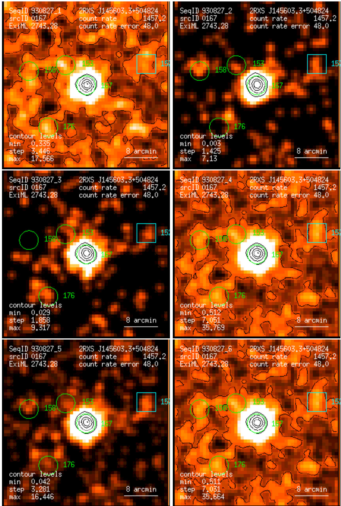
Figure 167: RASS 930827: detection 0167: band rate images, Gaussian filter: (1) PSPC channels 11 – 41, (2) 52 – 90, (3) 91 – 201, (4) 11 – 235, (5) 52 – 201, (6) 11 – 201. Broad band rates in counts/ks. Band rate contour levels in counts/ks/arcmin 2 .
