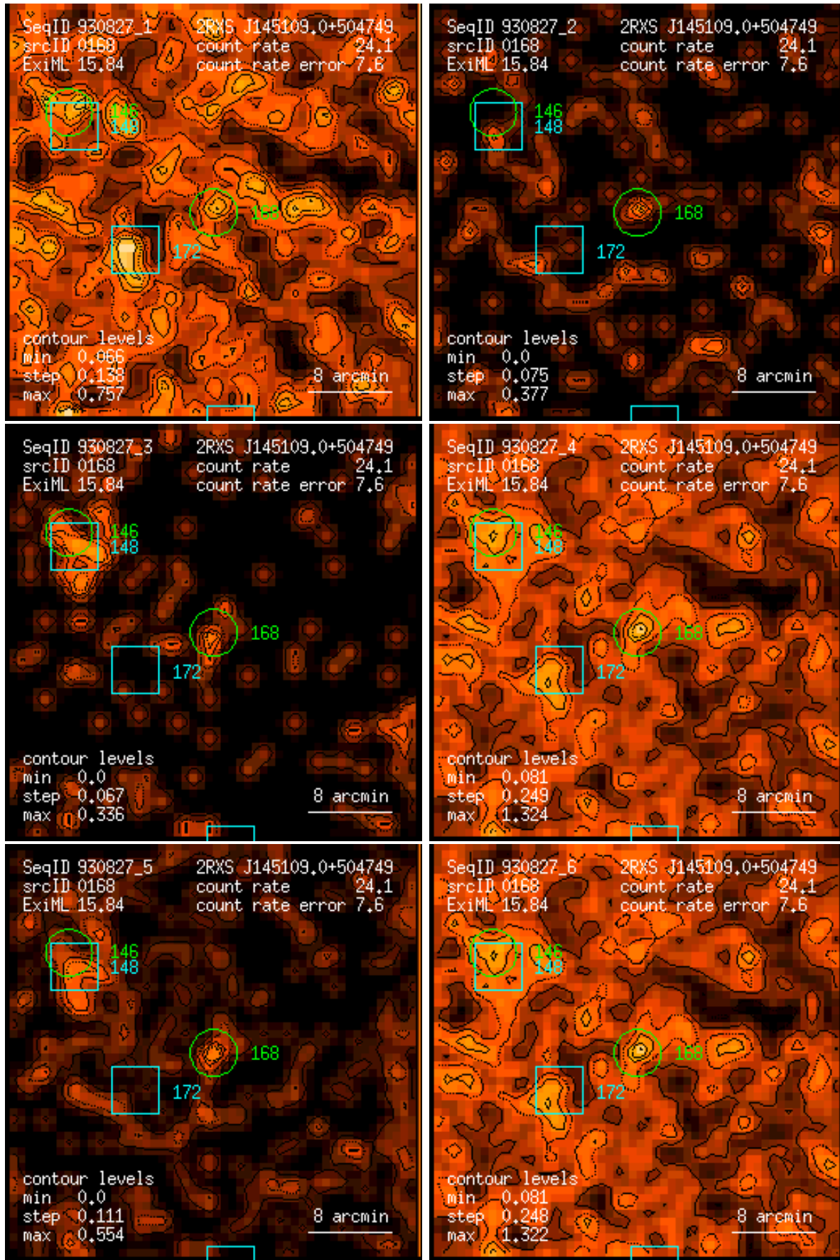
Figure 168: RASS 930827: detection 0168: band rate images, Gaussian filter: (1) PSPC channels 11 – 41, (2) 52 – 90, (3) 91 – 201, (4) 11 – 235, (5) 52 – 201, (6) 11 – 201. Broad band rates in counts/ks. Band rate contour levels in counts/ks/arcmin 2 .
