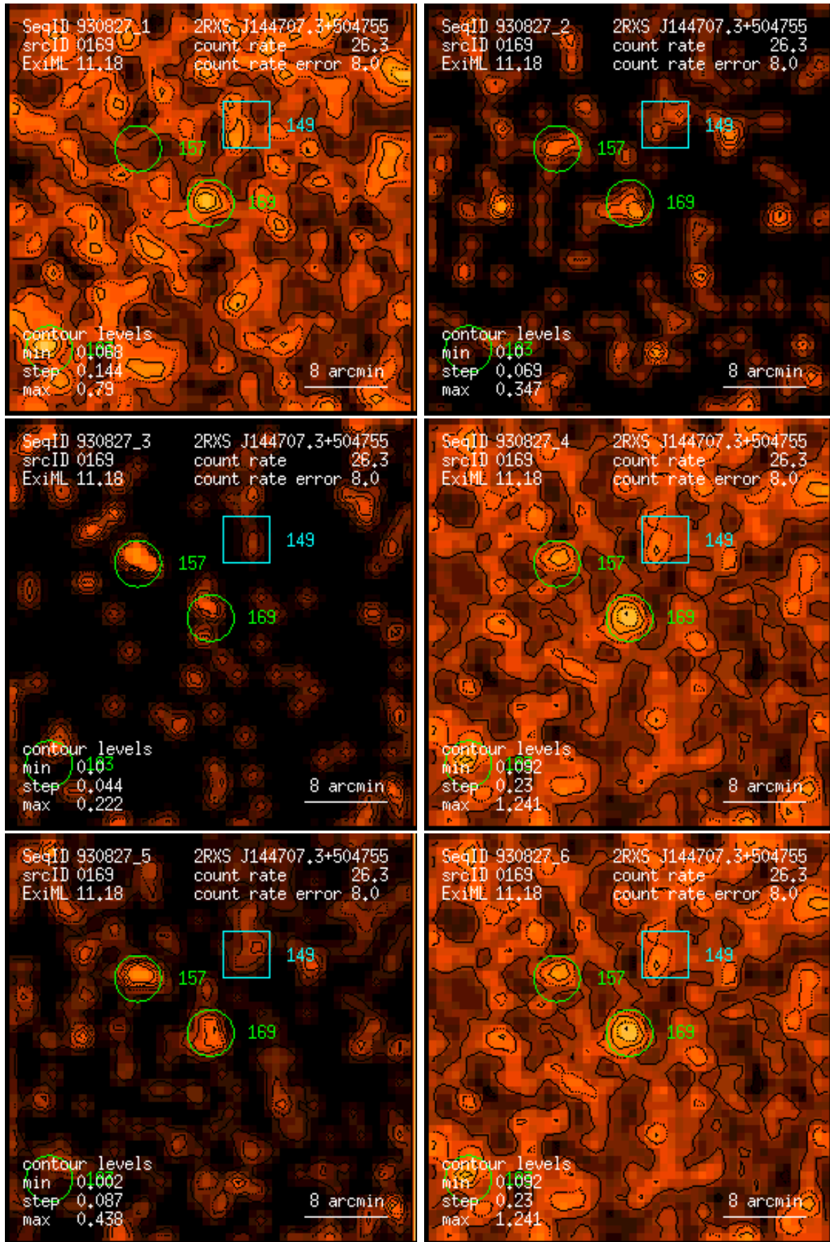
Figure 169: RASS 930827: detection 0169: band rate images, Gaussian filter: (1) PSPC channels 11 – 41, (2) 52 – 90, (3) 91 – 201, (4) 11 – 235, (5) 52 – 201, (6) 11 – 201. Broad band rates in counts/ks. Band rate contour levels in counts/ks/arcmin 2 .
