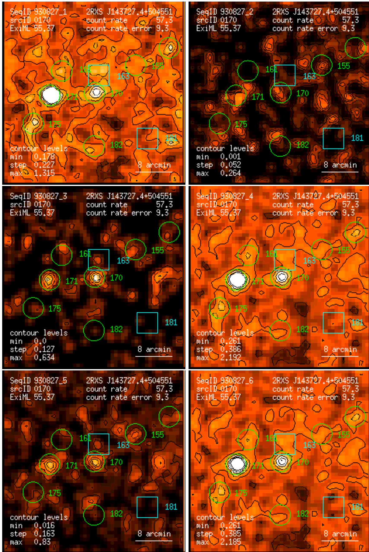
Figure 170: RASS 930827: detection 0170: band rate images, Gaussian filter: (1) PSPC channels 11 – 41, (2) 52 – 90, (3) 91 – 201, (4) 11 – 235, (5) 52 – 201, (6) 11 – 201. Broad band rates in counts/ks. Band rate contour levels in counts/ks/arcmin 2 .
