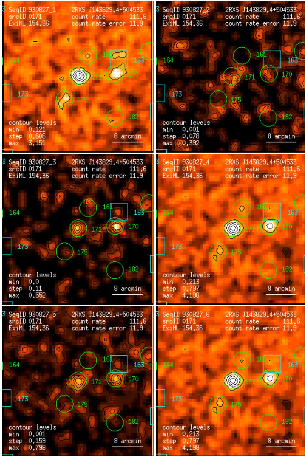
Figure 171: RASS 930827: detection 0171: band rate images, Gaussian filter: (1) PSPC channels 11 – 41, (2) 52 – 90, (3) 91 – 201, (4) 11 – 235, (5) 52 – 201, (6) 11 – 201. Broad band rates in counts/ks. Band rate contour levels in counts/ks/arcmin 2 .
