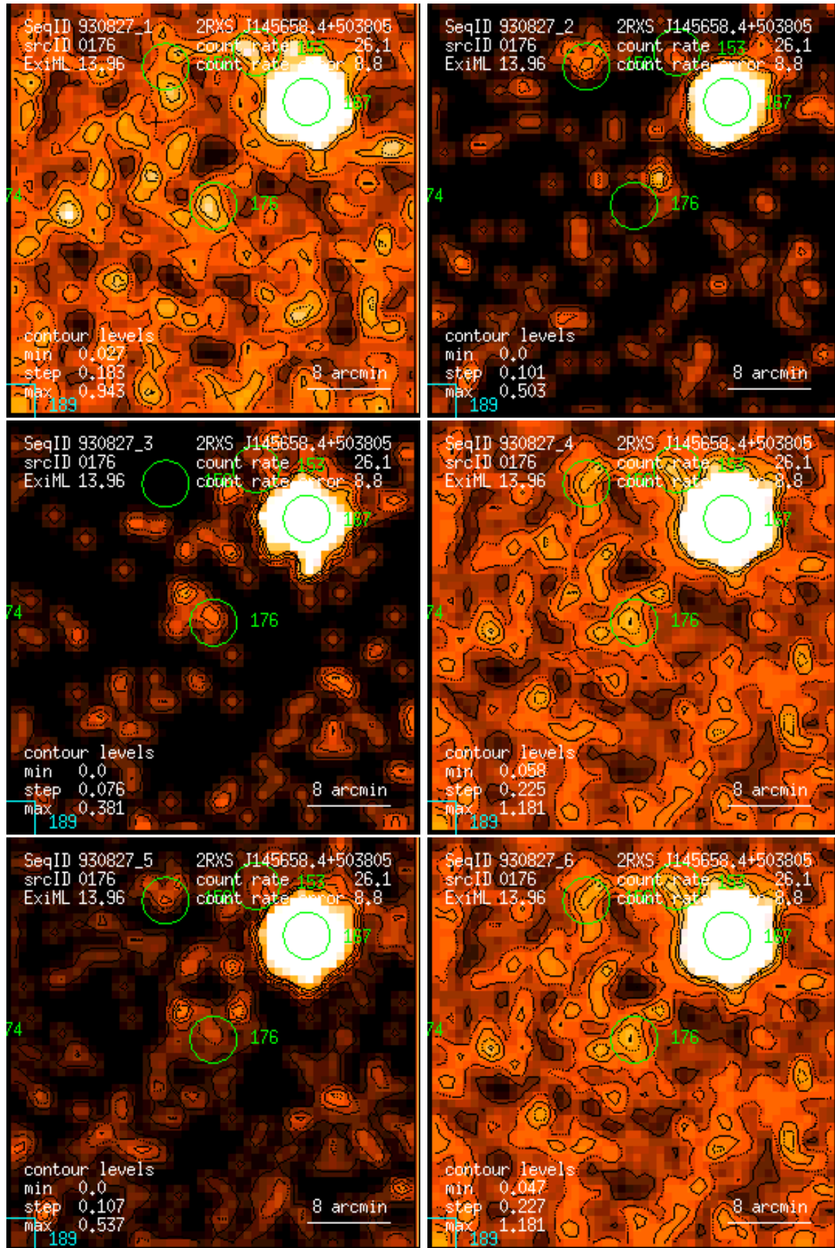
Figure 176: RASS 930827: detection 0176: band rate images, Gaussian filter: (1) PSPC channels 11 – 41, (2) 52 – 90, (3) 91 – 201, (4) 11 – 235, (5) 52 – 201, (6) 11 – 201. Broad band rates in counts/ks. Band rate contour levels in counts/ks/arcmin 2 .
