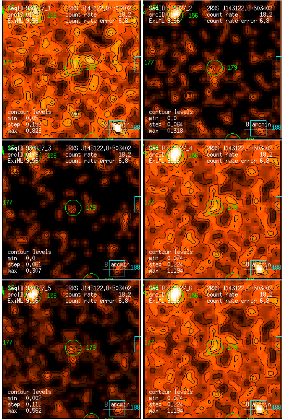
Figure 179: RASS 930827: detection 0179: band rate images, Gaussian filter: (1) PSPC channels 11 – 41, (2) 52 – 90, (3) 91 – 201, (4) 11 – 235, (5) 52 – 201, (6) 11 – 201. Broad band rates in counts/ks. Band rate contour levels in counts/ks/arcmin 2 .
