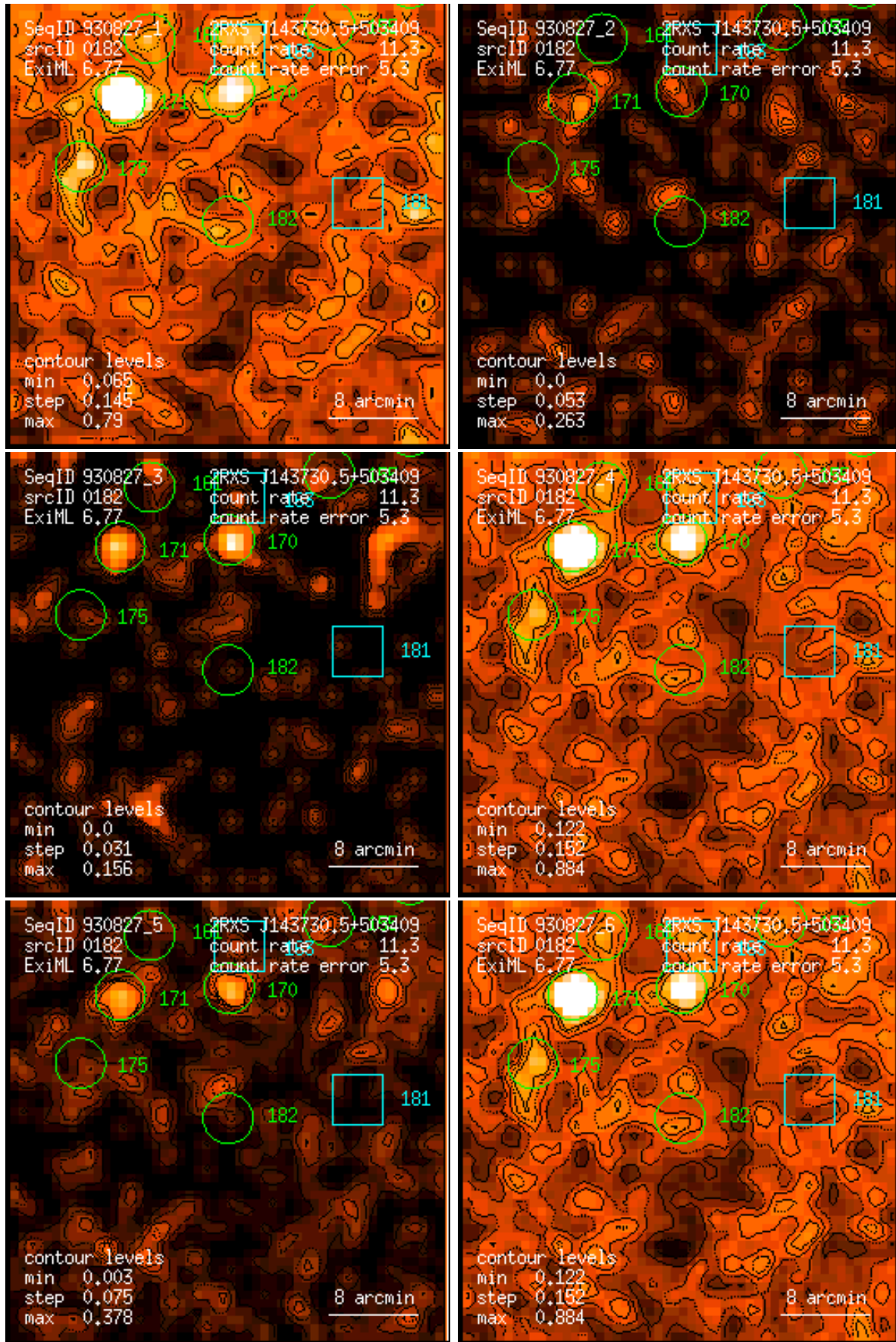
Figure 182: RASS 930827: detection 0182: band rate images, Gaussian filter: (1) PSPC channels 11 – 41, (2) 52 – 90, (3) 91 – 201, (4) 11 – 235, (5) 52 – 201, (6) 11 – 201. Broad band rates in counts/ks. Band rate contour levels in counts/ks/arcmin 2 .
