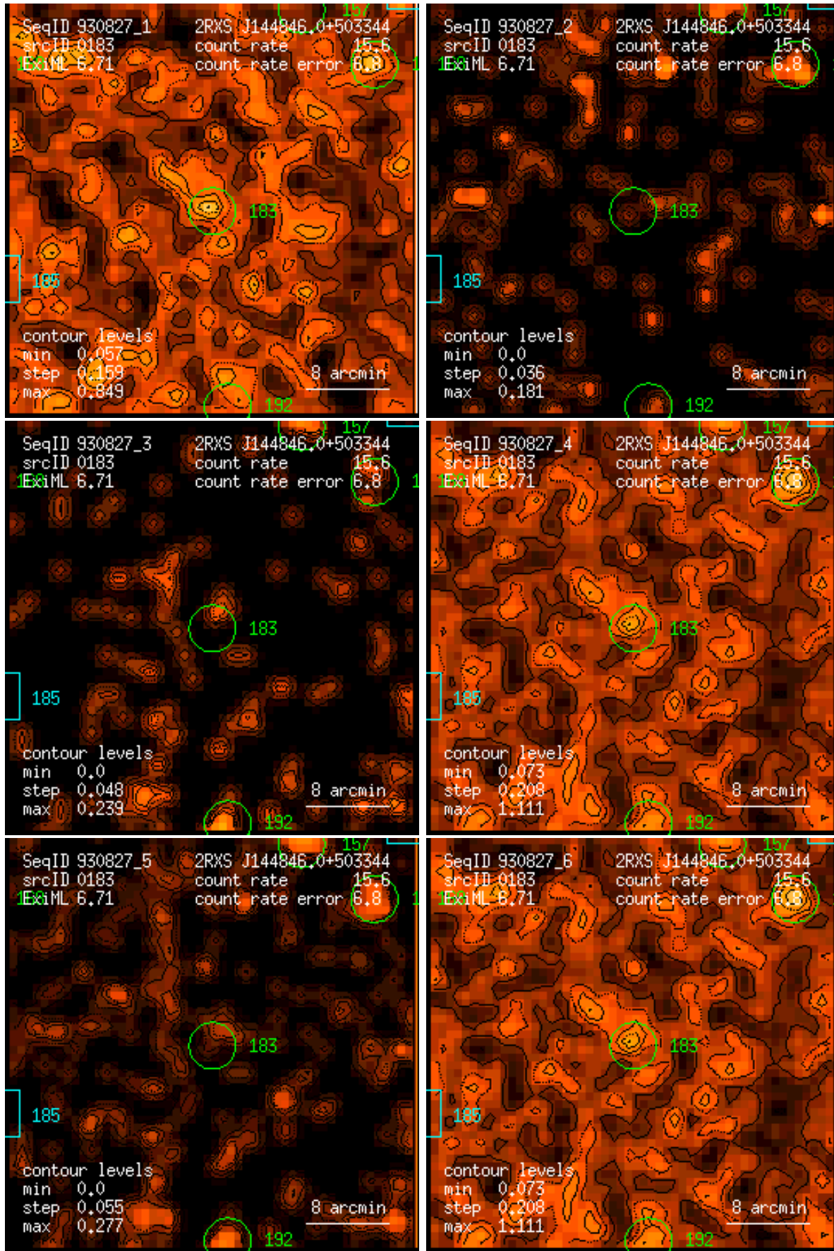
Figure 183: RASS 930827: detection 0183: band rate images, Gaussian filter: (1) PSPC channels 11 – 41, (2) 52 – 90, (3) 91 – 201, (4) 11 – 235, (5) 52 – 201, (6) 11 – 201. Broad band rates in counts/ks. Band rate contour levels in counts/ks/arcmin 2 .
