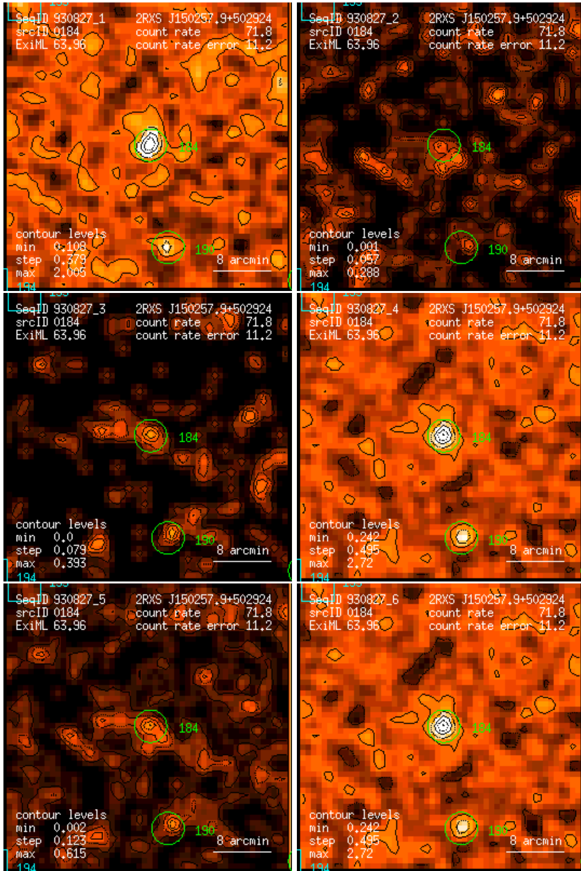
Figure 184: RASS 930827: detection 0184: band rate images, Gaussian filter: (1) PSPC channels 11 – 41, (2) 52 – 90, (3) 91 – 201, (4) 11 – 235, (5) 52 – 201, (6) 11 – 201. Broad band rates in counts/ks. Band rate contour levels in counts/ks/arcmin 2 .
