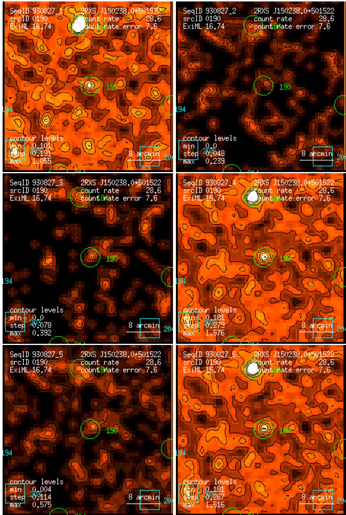
Figure 190: RASS 930827: detection 0190: band rate images, Gaussian filter: (1) PSPC channels 11 – 41, (2) 52 – 90, (3) 91 – 201, (4) 11 – 235, (5) 52 – 201, (6) 11 – 201. Broad band rates in counts/ks. Band rate contour levels in counts/ks/arcmin 2 .
