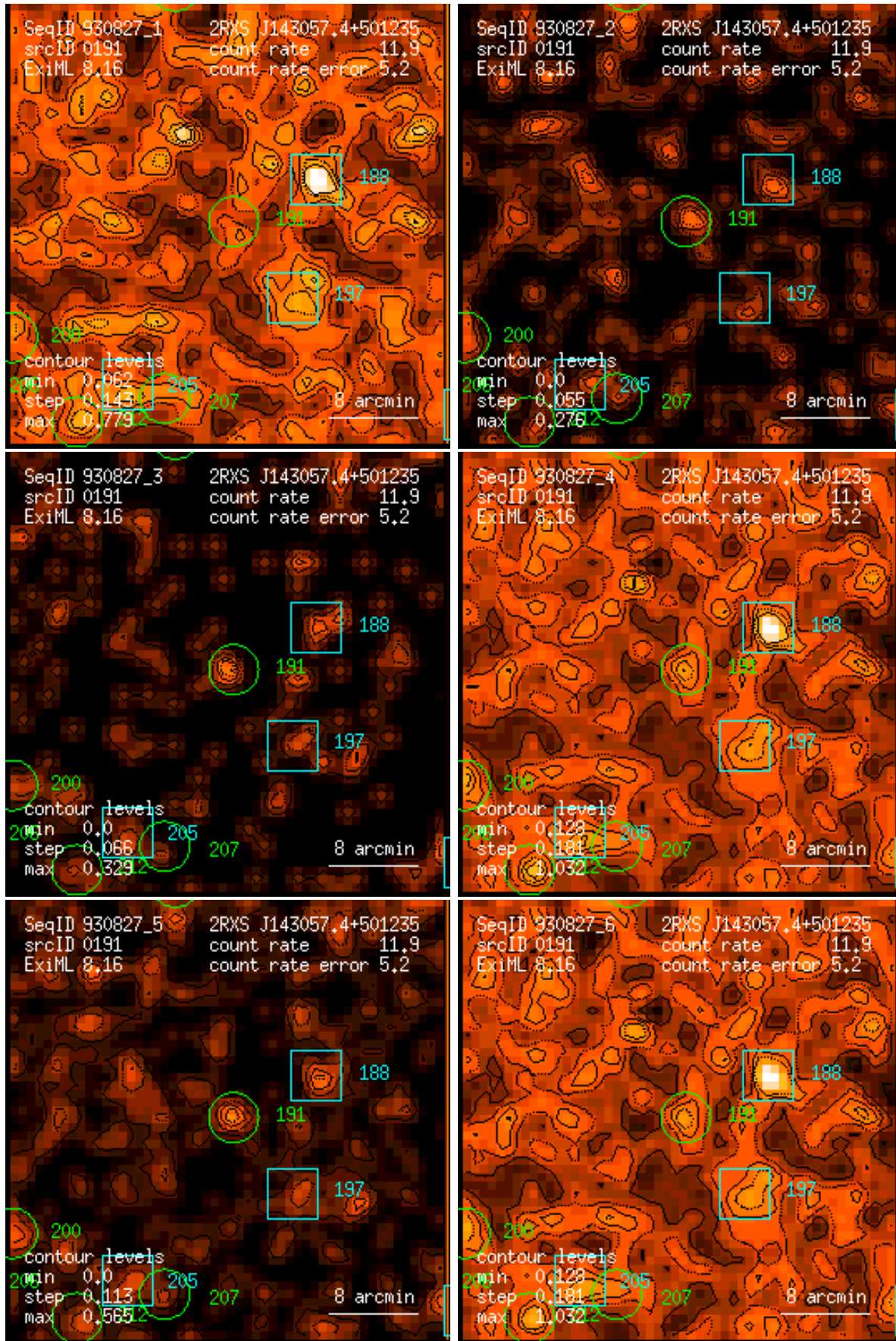
Figure 191: RASS 930827: detection 0191: band rate images, Gaussian filter: (1) PSPC channels 11 – 41, (2) 52 – 90, (3) 91 – 201, (4) 11 – 235, (5) 52 – 201, (6) 11 – 201. Broad band rates in counts/ks. Band rate contour levels in counts/ks/arcmin 2 .
