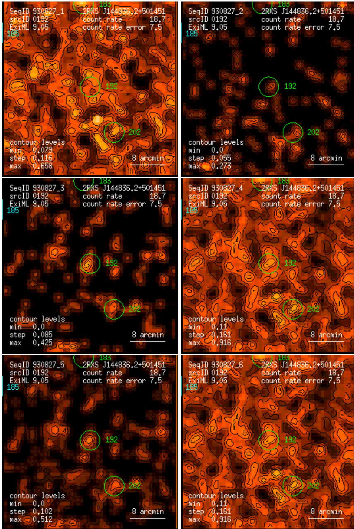
Figure 192: RASS 930827: detection 0192: band rate images, Gaussian filter: (1) PSPC channels 11 – 41, (2) 52 – 90, (3) 91 – 201, (4) 11 – 235, (5) 52 – 201, (6) 11 – 201. Broad band rates in counts/ks. Band rate contour levels in counts/ks/arcmin 2 .
