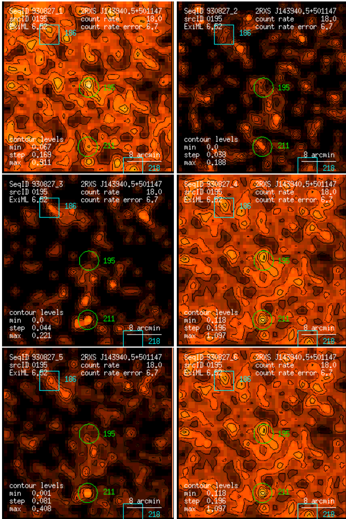
Figure 195: RASS 930827: detection 0195: band rate images, Gaussian filter: (1) PSPC channels 11 – 41, (2) 52 – 90, (3) 91 – 201, (4) 11 – 235, (5) 52 – 201, (6) 11 – 201. Broad band rates in counts/ks. Band rate contour levels in counts/ks/arcmin 2 .
