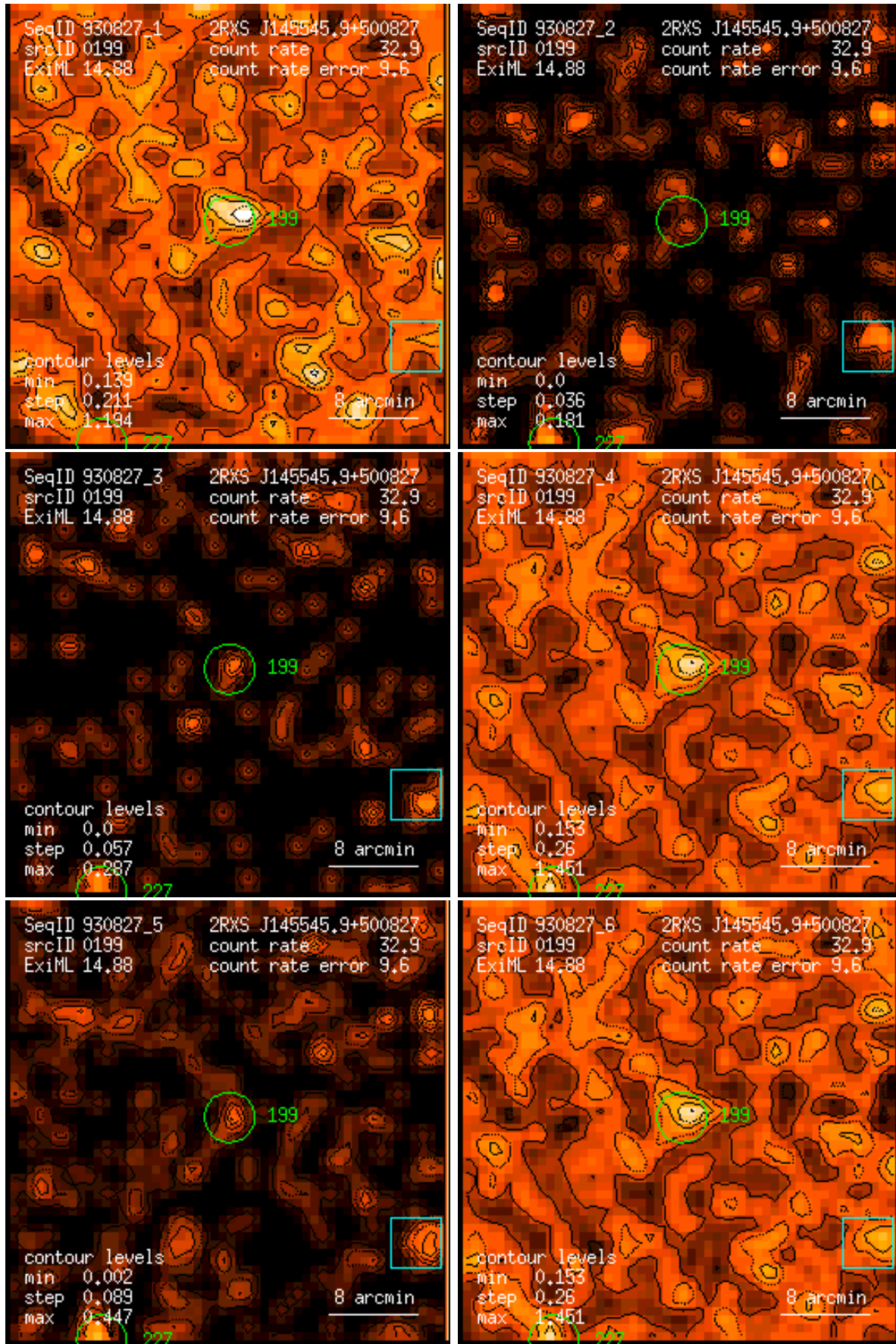
Figure 199: RASS 930827: detection 0199: band rate images, Gaussian filter: (1) PSPC channels 11 – 41, (2) 52 – 90, (3) 91 – 201, (4) 11 – 235, (5) 52 – 201, (6) 11 – 201. Broad band rates in counts/ks. Band rate contour levels in counts/ks/arcmin 2 .
