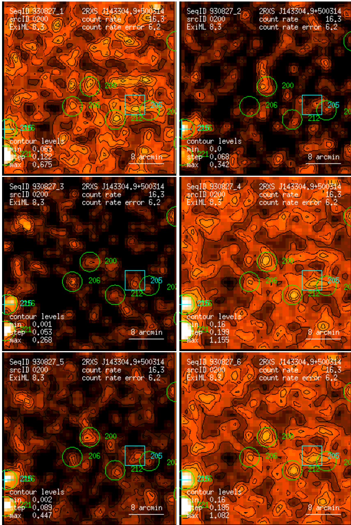
Figure 200: RASS 930827: detection 0200: band rate images, Gaussian filter: (1) PSPC channels 11 – 41, (2) 52 – 90, (3) 91 – 201, (4) 11 – 235, (5) 52 – 201, (6) 11 – 201. Broad band rates in counts/ks. Band rate contour levels in counts/ks/arcmin 2 .
