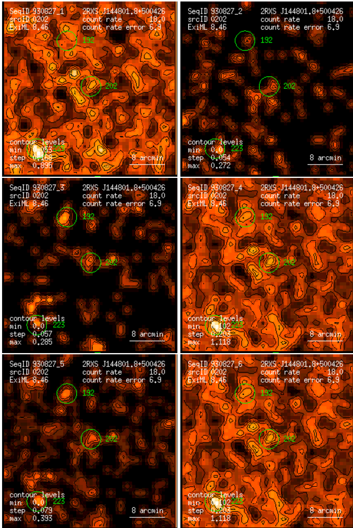
Figure 202: RASS 930827: detection 0202: band rate images, Gaussian filter: (1) PSPC channels 11 – 41, (2) 52 – 90, (3) 91 – 201, (4) 11 – 235, (5) 52 – 201, (6) 11 – 201. Broad band rates in counts/ks. Band rate contour levels in counts/ks/arcmin 2 .
