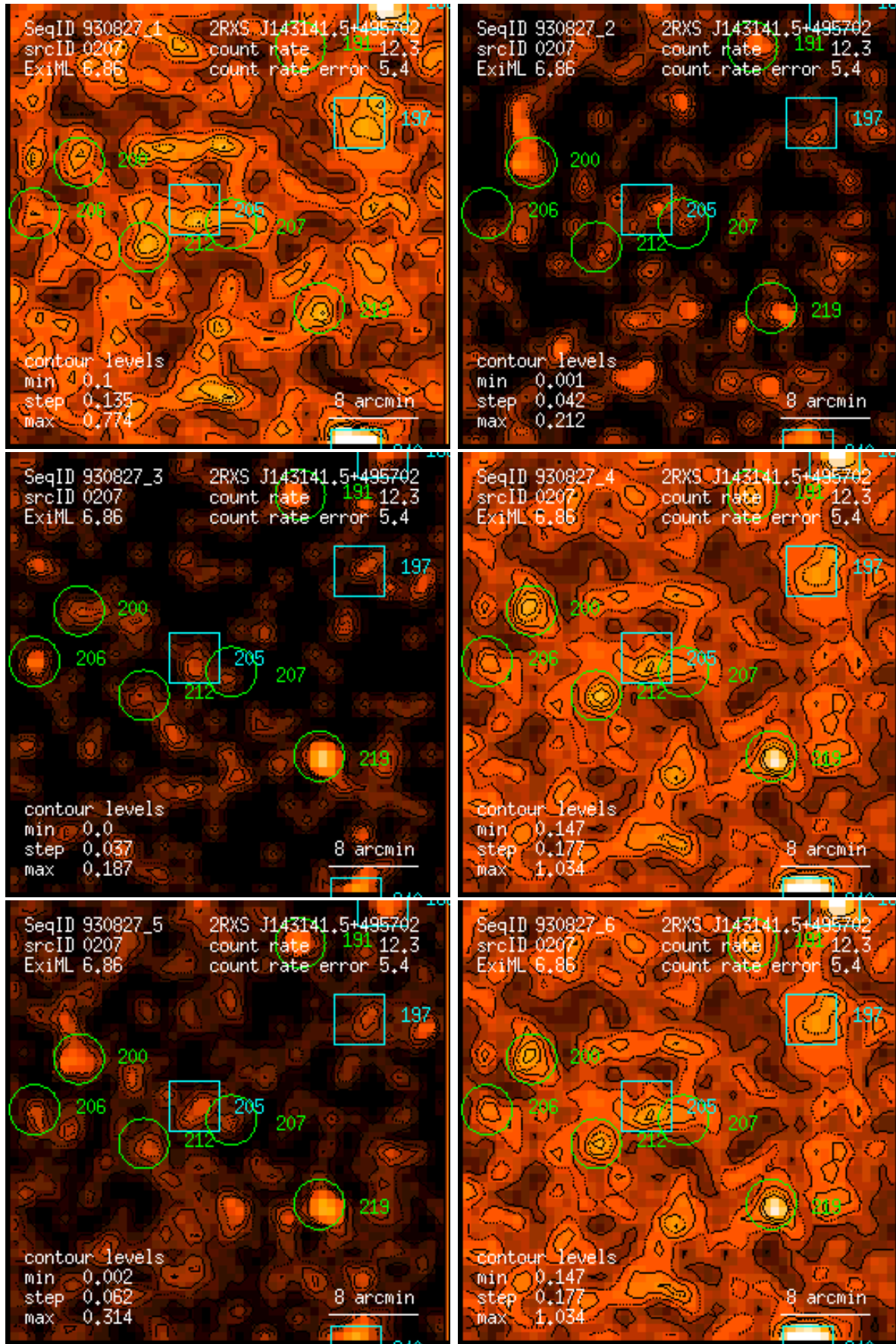
Figure 207: RASS 930827: detection 0207: band rate images, Gaussian filter: (1) PSPC channels 11 – 41, (2) 52 – 90, (3) 91 – 201, (4) 11 – 235, (5) 52 – 201, (6) 11 – 201. Broad band rates in counts/ks. Band rate contour levels in counts/ks/arcmin 2 .
