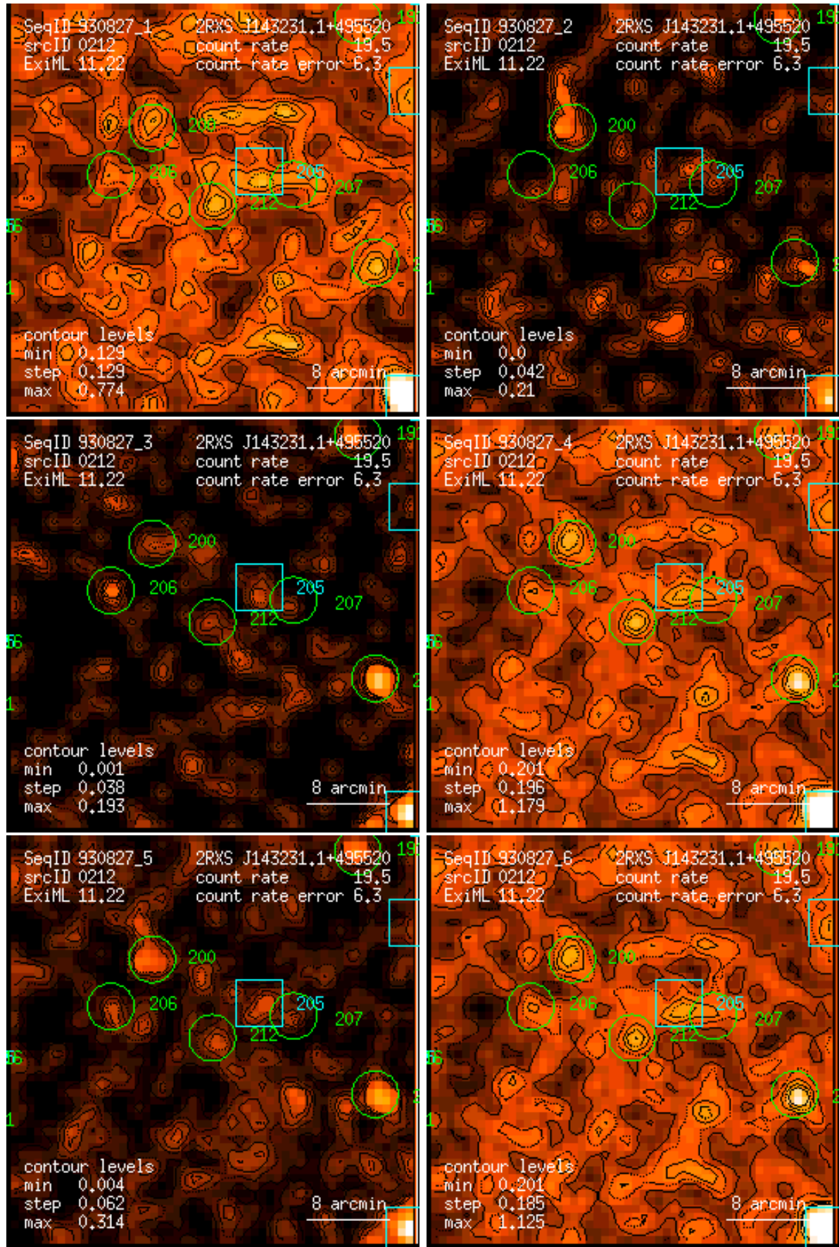
Figure 212: RASS 930827: detection 0212: band rate images, Gaussian filter: (1) PSPC channels 11 – 41, (2) 52 – 90, (3) 91 – 201, (4) 11 – 235, (5) 52 – 201, (6) 11 – 201. Broad band rates in counts/ks. Band rate contour levels in counts/ks/arcmin 2 .
