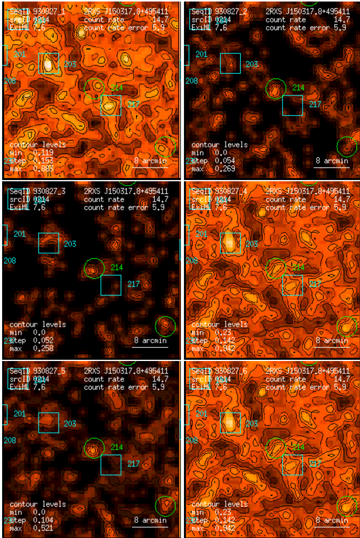
Figure 214: RASS 930827: detection 0214: band rate images, Gaussian filter: (1) PSPC channels 11 – 41, (2) 52 – 90, (3) 91 – 201, (4) 11 – 235, (5) 52 – 201, (6) 11 – 201. Broad band rates in counts/ks. Band rate contour levels in counts/ks/arcmin 2 .
