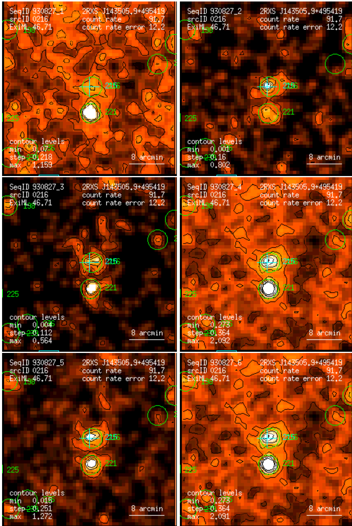
Figure 216: RASS 930827: detection 0216: band rate images, Gaussian filter: (1) PSPC channels 11 – 41, (2) 52 – 90, (3) 91 – 201, (4) 11 – 235, (5) 52 – 201, (6) 11 – 201. Broad band rates in counts/ks. Band rate contour levels in counts/ks/arcmin 2 .
