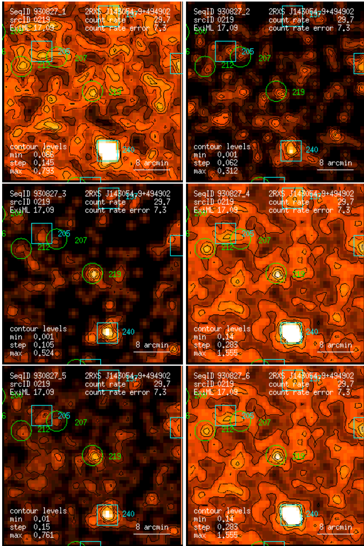
Figure 219: RASS 930827: detection 0219: band rate images, Gaussian filter: (1) PSPC channels 11 – 41, (2) 52 – 90, (3) 91 – 201, (4) 11 – 235, (5) 52 – 201, (6) 11 – 201. Broad band rates in counts/ks. Band rate contour levels in counts/ks/arcmin 2 .
