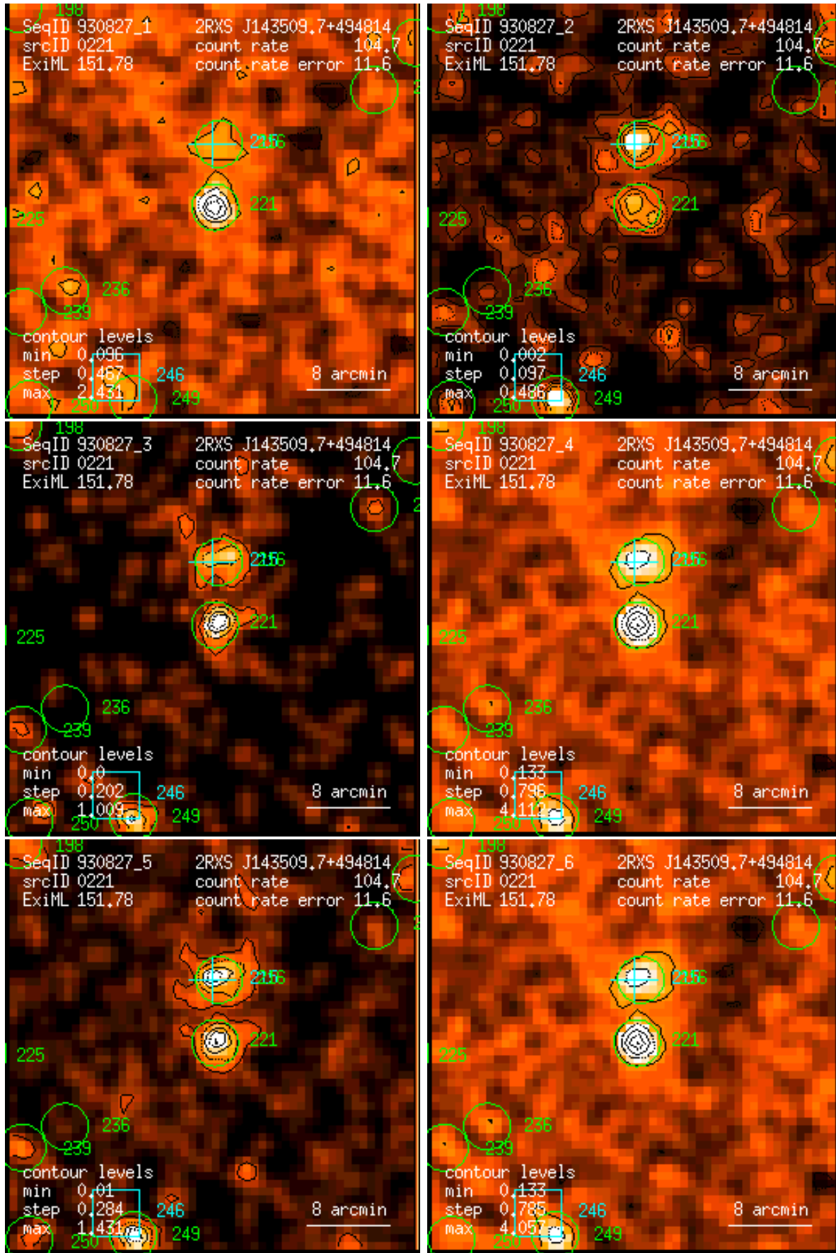
Figure 221: RASS 930827: detection 0221: band rate images, Gaussian filter: (1) PSPC channels 11 – 41, (2) 52 – 90, (3) 91 – 201, (4) 11 – 235, (5) 52 – 201, (6) 11 – 201. Broad band rates in counts/ks. Band rate contour levels in counts/ks/arcmin 2 .
