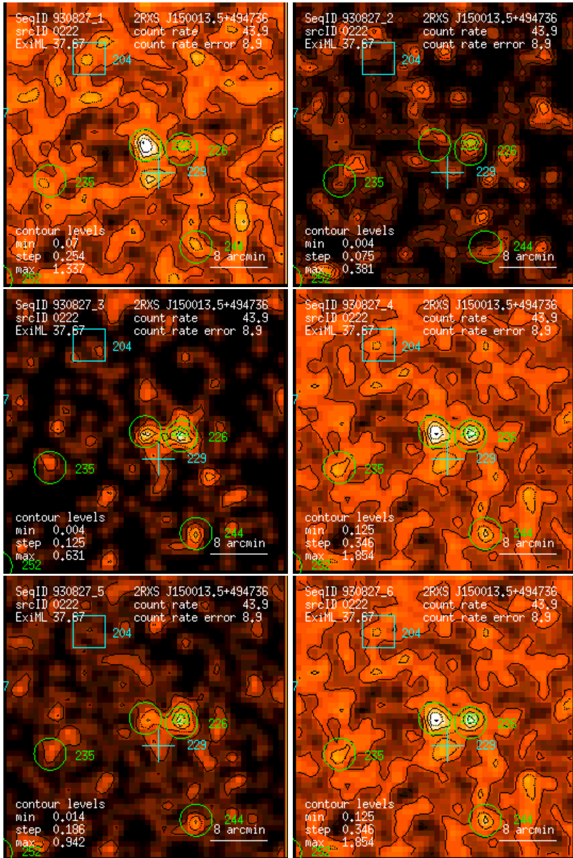
Figure 222: RASS 930827: detection 0222: band rate images, Gaussian filter: (1) PSPC channels 11 – 41, (2) 52 – 90, (3) 91 – 201, (4) 11 – 235, (5) 52 – 201, (6) 11 – 201. Broad band rates in counts/ks. Band rate contour levels in counts/ks/arcmin 2 .
