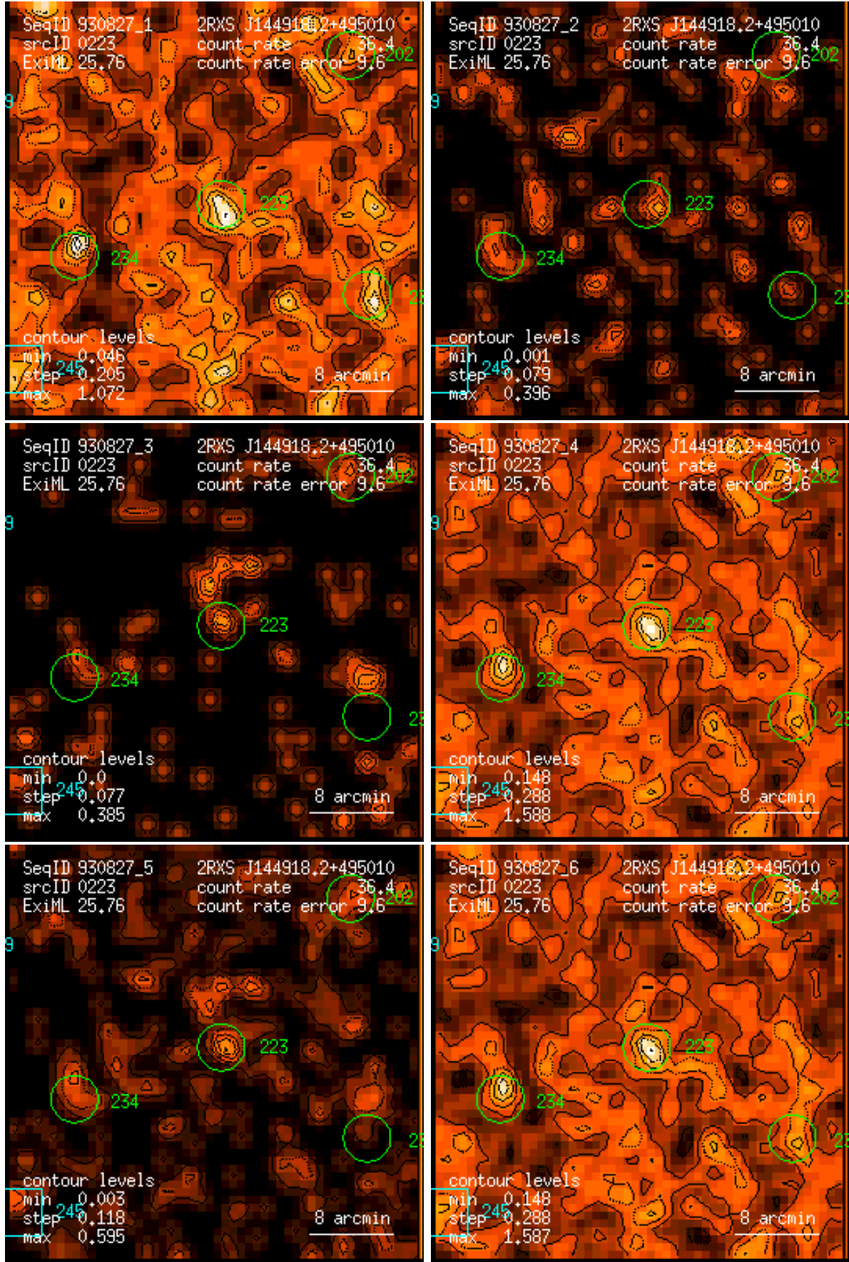
Figure 223: RASS 930827: detection 0223: band rate images, Gaussian filter: (1) PSPC channels 11 – 41, (2) 52 – 90, (3) 91 – 201, (4) 11 – 235, (5) 52 – 201, (6) 11 – 201. Broad band rates in counts/ks. Band rate contour levels in counts/ks/arcmin 2 .
