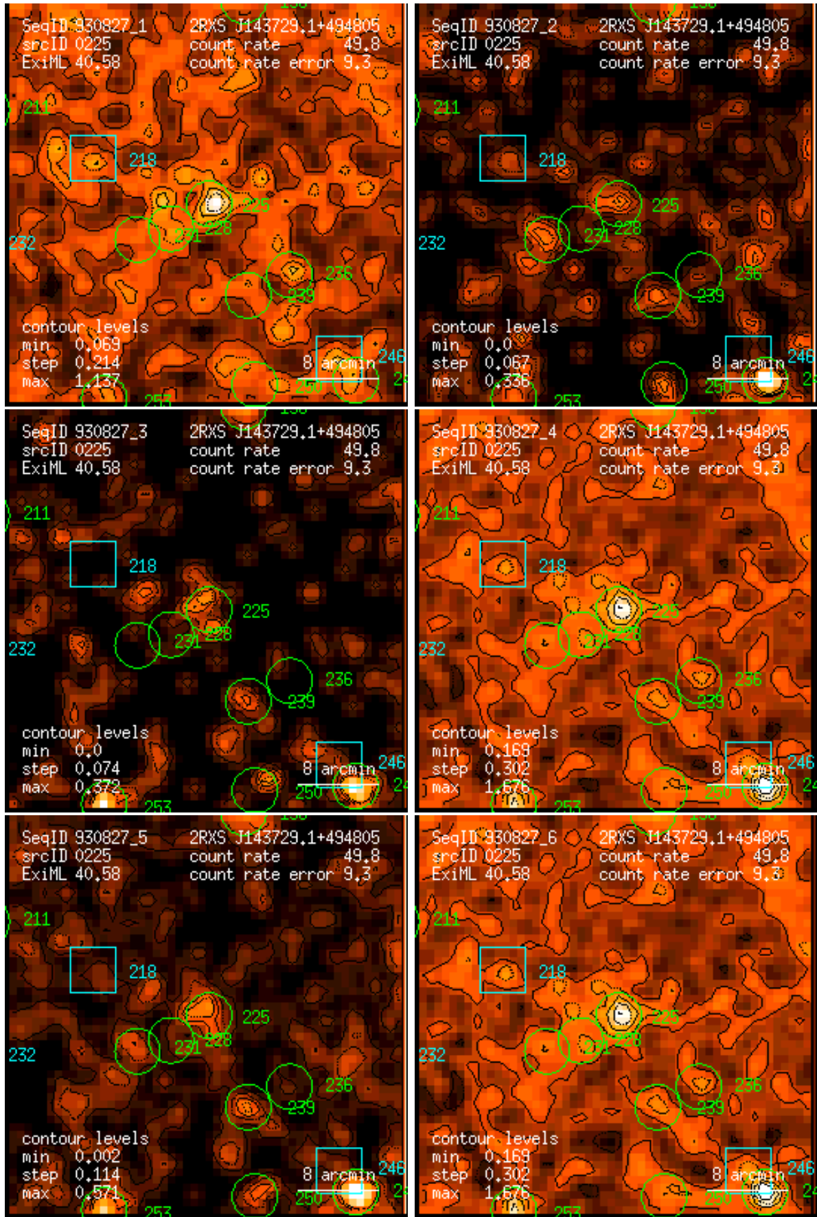
Figure 225: RASS 930827: detection 0225: band rate images, Gaussian filter: (1) PSPC channels 11 – 41, (2) 52 – 90, (3) 91 – 201, (4) 11 – 235, (5) 52 – 201, (6) 11 – 201. Broad band rates in counts/ks. Band rate contour levels in counts/ks/arcmin 2 .
