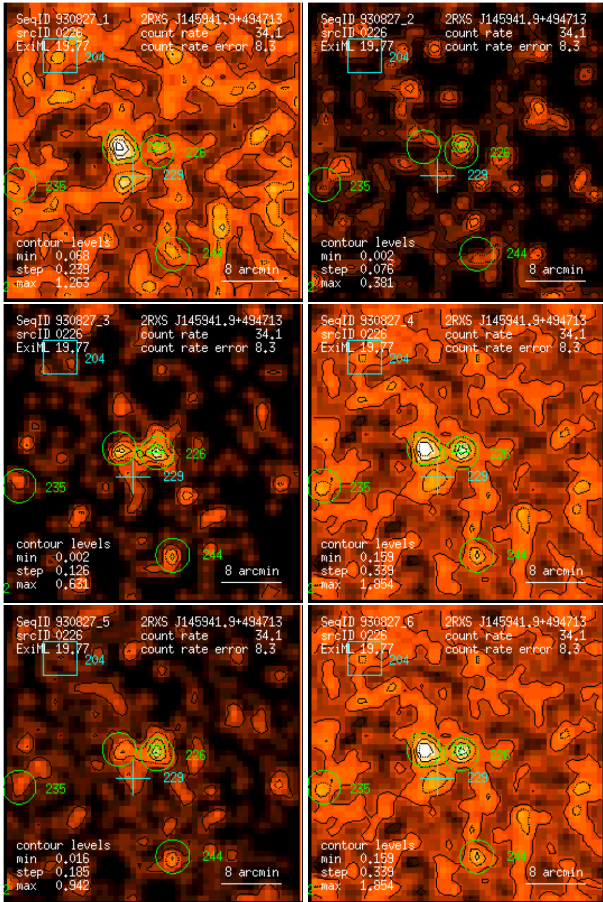
Figure 226: RASS 930827: detection 0226: band rate images, Gaussian filter: (1) PSPC channels 11 – 41, (2) 52 – 90, (3) 91 – 201, (4) 11 – 235, (5) 52 – 201, (6) 11 – 201. Broad band rates in counts/ks. Band rate contour levels in counts/ks/arcmin 2 .
