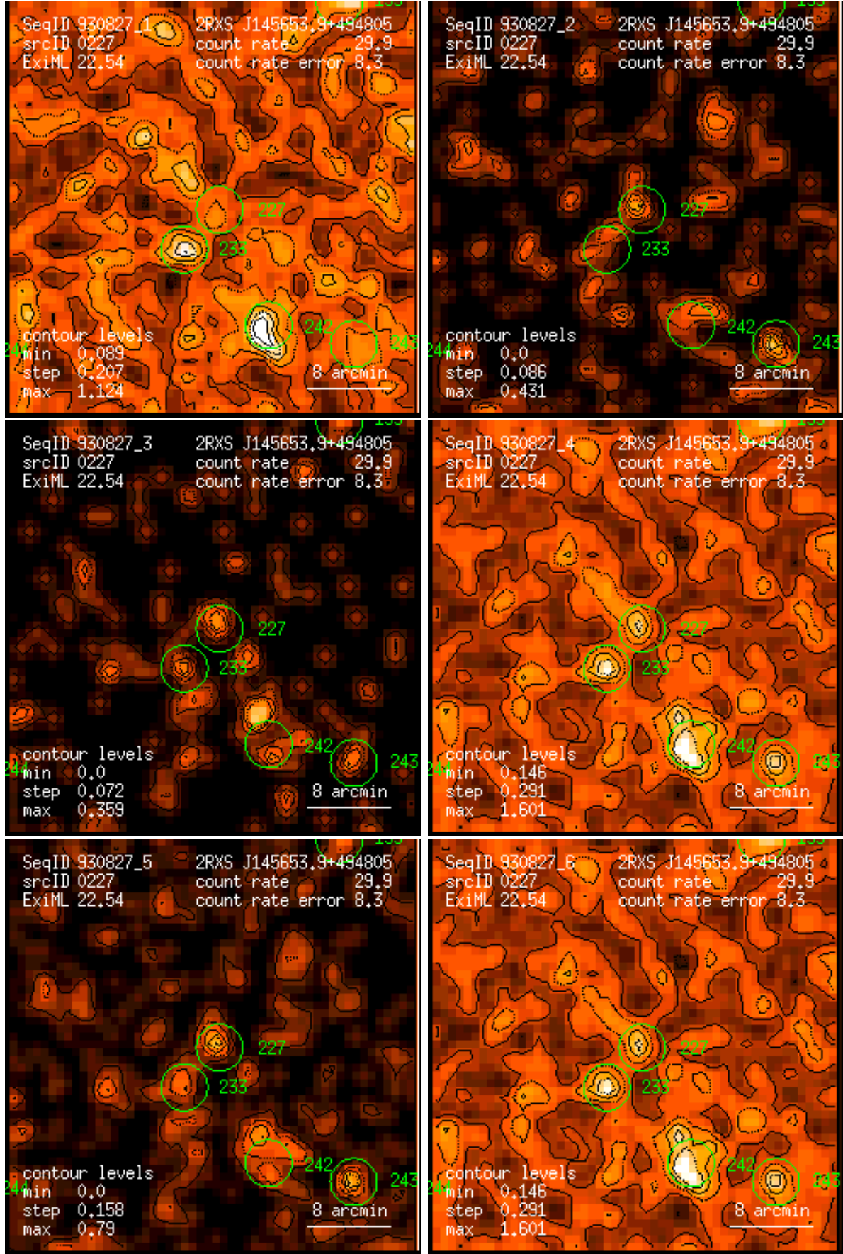
Figure 227: RASS 930827: detection 0227: band rate images, Gaussian filter: (1) PSPC channels 11 – 41, (2) 52 – 90, (3) 91 – 201, (4) 11 – 235, (5) 52 – 201, (6) 11 – 201. Broad band rates in counts/ks. Band rate contour levels in counts/ks/arcmin 2 .
