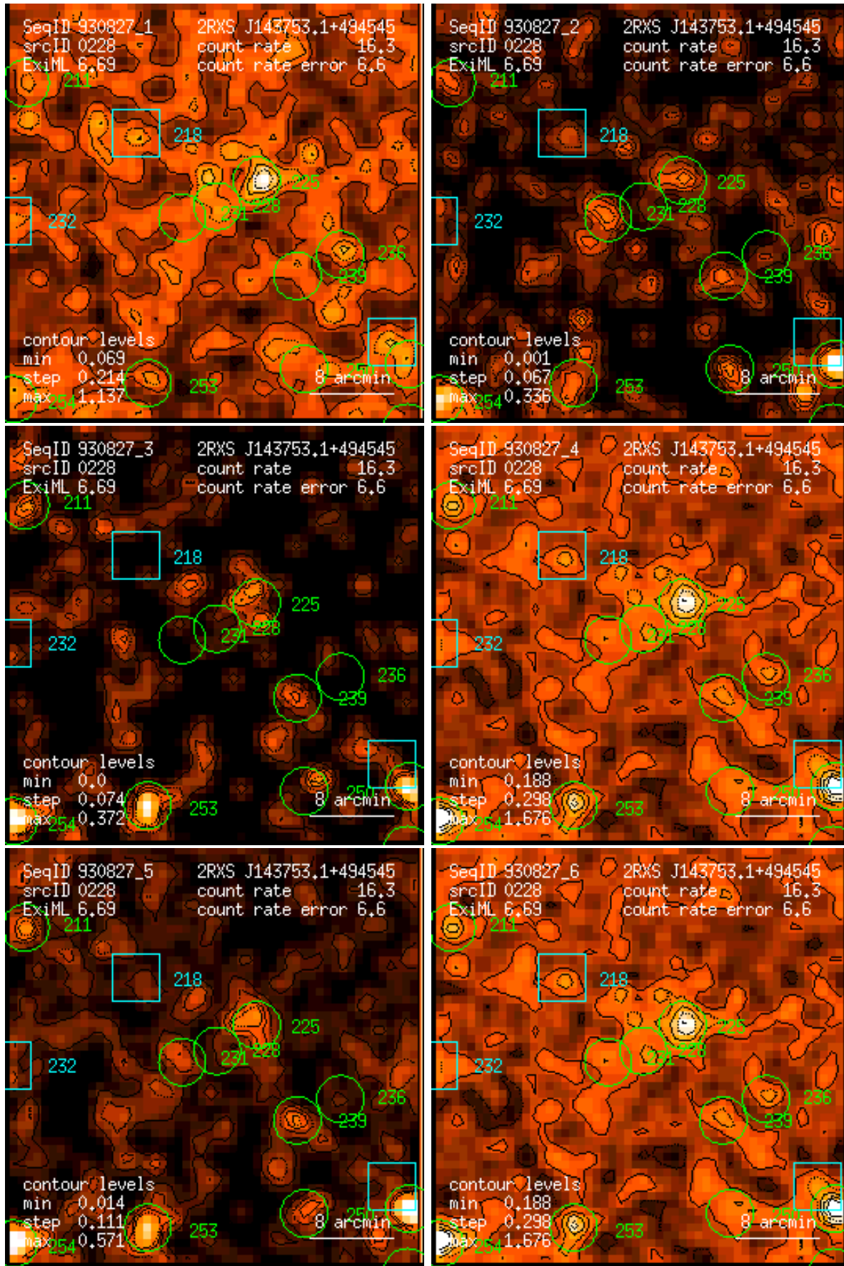
Figure 228: RASS 930827: detection 0228: band rate images, Gaussian filter: (1) PSPC channels 11 – 41, (2) 52 – 90, (3) 91 – 201, (4) 11 – 235, (5) 52 – 201, (6) 11 – 201. Broad band rates in counts/ks. Band rate contour levels in counts/ks/arcmin 2 .
