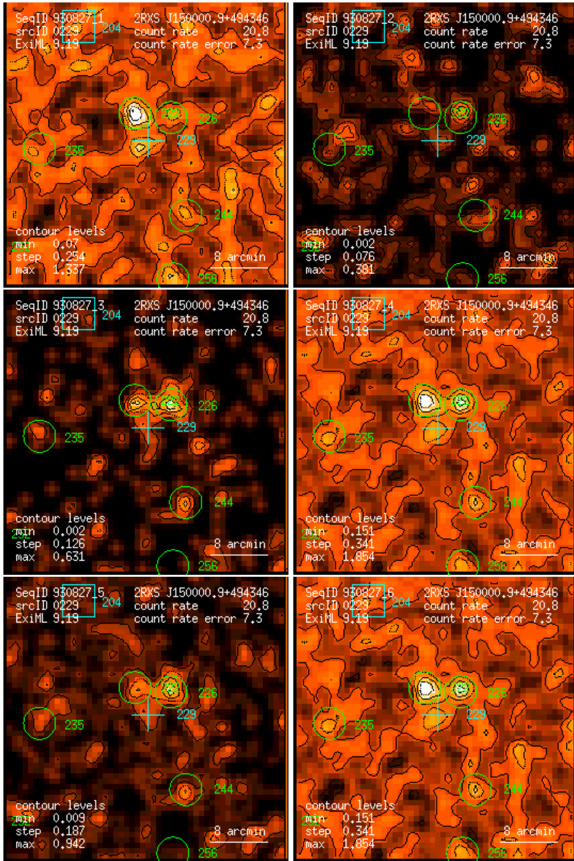
Figure 229: RASS 930827: detection 0229: band rate images, Gaussian filter: (1) PSPC channels 11 – 41, (2) 52 – 90, (3) 91 – 201, (4) 11 – 235, (5) 52 – 201, (6) 11 – 201. Broad band rates in counts/ks. Band rate contour levels in counts/ks/arcmin 2 .
