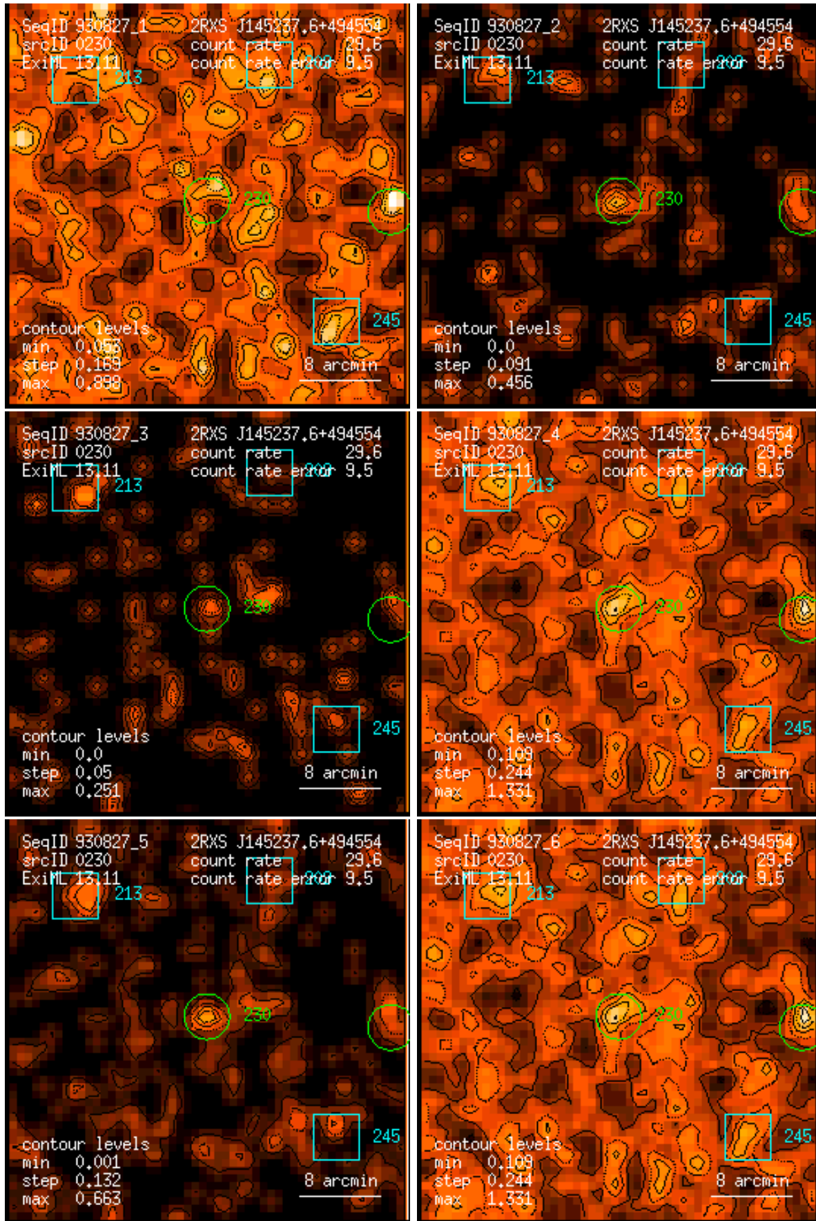
Figure 230: RASS 930827: detection 0230: band rate images, Gaussian filter: (1) PSPC channels 11 – 41, (2) 52 – 90, (3) 91 – 201, (4) 11 – 235, (5) 52 – 201, (6) 11 – 201. Broad band rates in counts/ks. Band rate contour levels in counts/ks/arcmin 2 .
