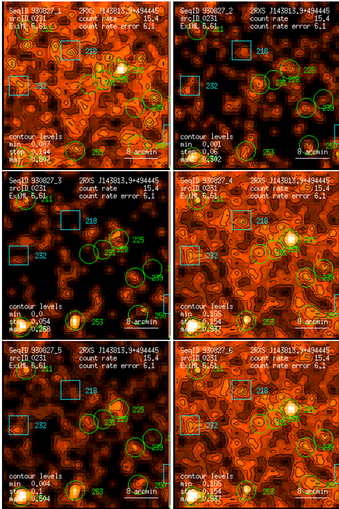
Figure 231: RASS 930827: detection 0231: band rate images, Gaussian filter: (1) PSPC channels 11 – 41, (2) 52 – 90, (3) 91 – 201, (4) 11 – 235, (5) 52 – 201, (6) 11 – 201. Broad band rates in counts/ks. Band rate contour levels in counts/ks/arcmin 2 .
