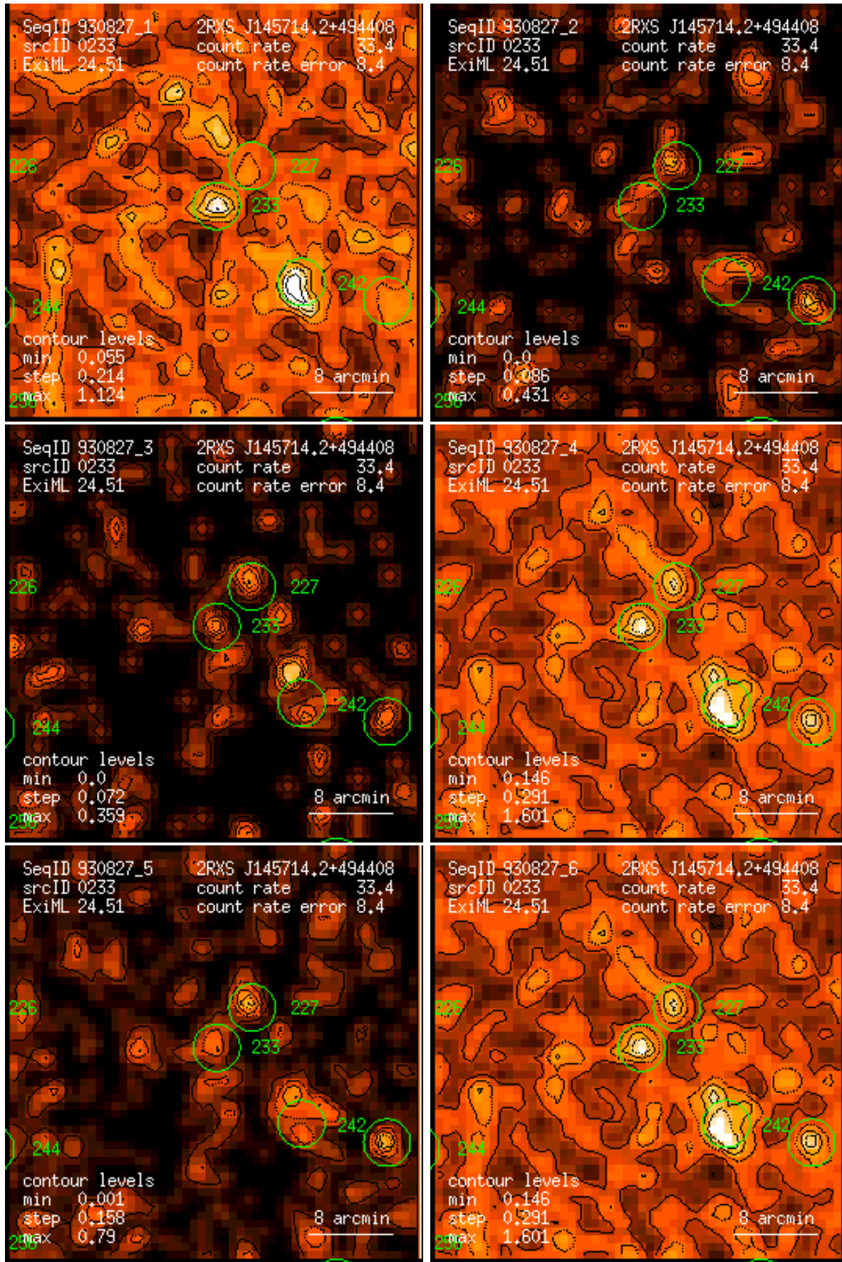
Figure 233: RASS 930827: detection 0233: band rate images, Gaussian filter: (1) PSPC channels 11 – 41, (2) 52 – 90, (3) 91 – 201, (4) 11 – 235, (5) 52 – 201, (6) 11 – 201. Broad band rates in counts/ks. Band rate contour levels in counts/ks/arcmin 2 .
