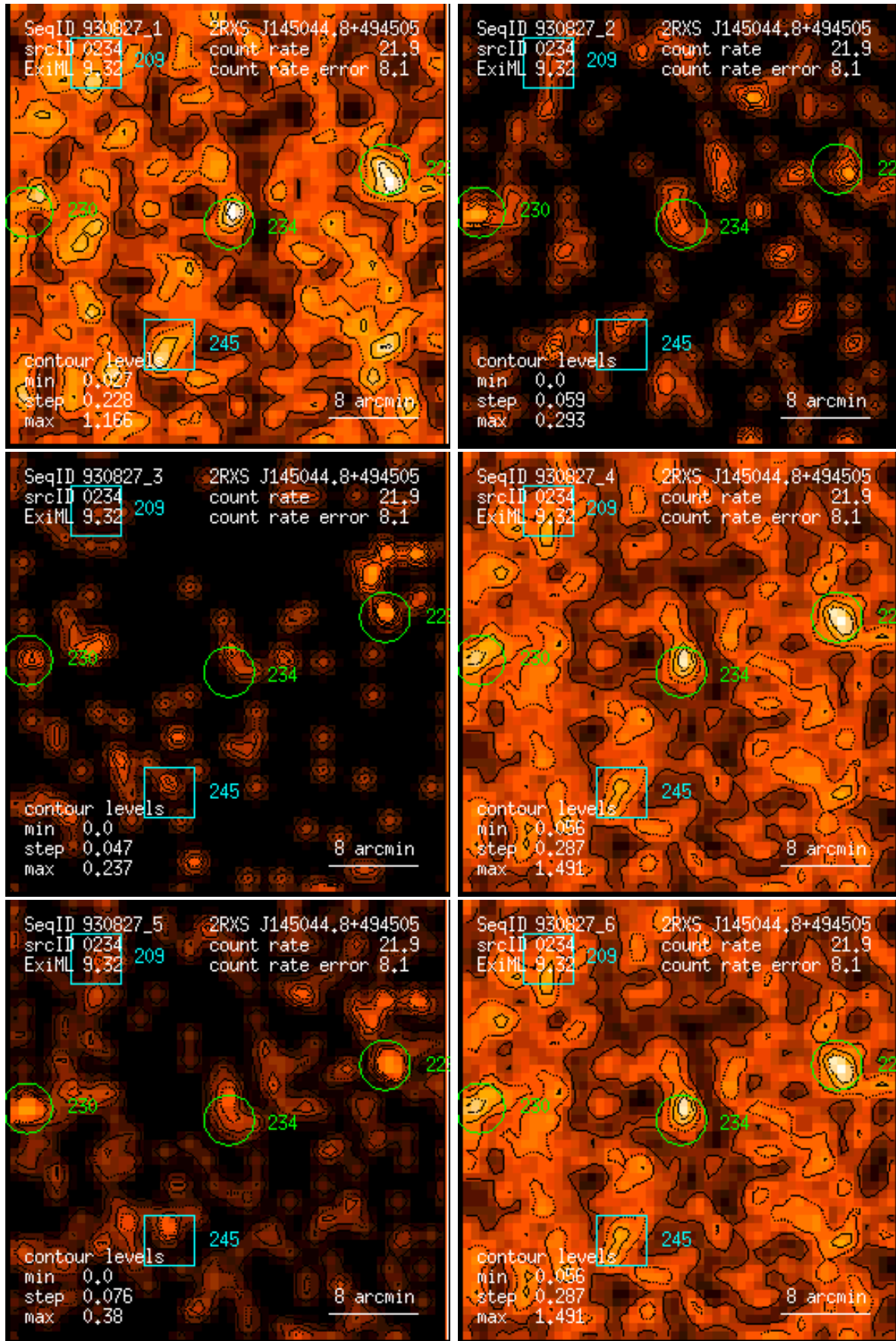
Figure 234: RASS 930827: detection 0234: band rate images, Gaussian filter: (1) PSPC channels 11 – 41, (2) 52 – 90, (3) 91 – 201, (4) 11 – 235, (5) 52 – 201, (6) 11 – 201. Broad band rates in counts/ks. Band rate contour levels in counts/ks/arcmin 2 .
