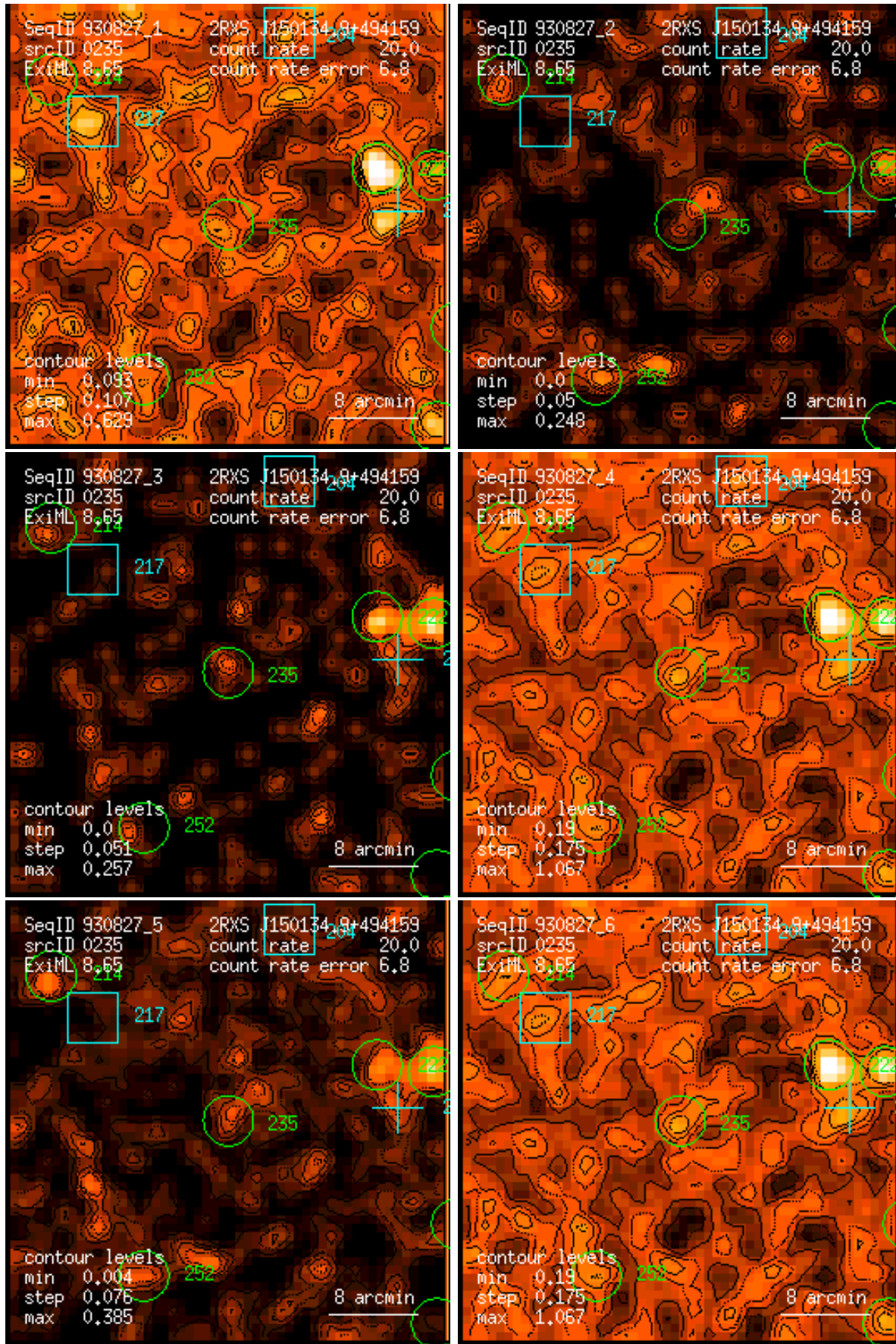
Figure 235: RASS 930827: detection 0235: band rate images, Gaussian filter: (1) PSPC channels 11 – 41, (2) 52 – 90, (3) 91 – 201, (4) 11 – 235, (5) 52 – 201, (6) 11 – 201. Broad band rates in counts/ks. Band rate contour levels in counts/ks/arcmin 2 .
