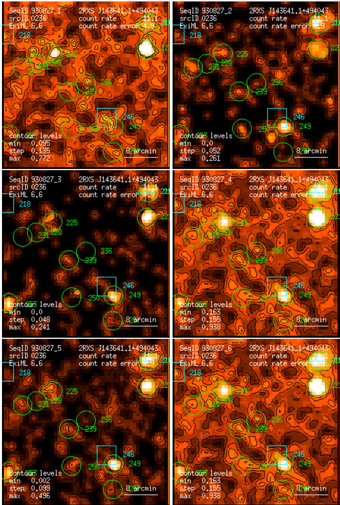
Figure 236: RASS 930827: detection 0236: band rate images, Gaussian filter: (1) PSPC channels 11 – 41, (2) 52 – 90, (3) 91 – 201, (4) 11 – 235, (5) 52 – 201, (6) 11 – 201. Broad band rates in counts/ks. Band rate contour levels in counts/ks/arcmin 2 .
